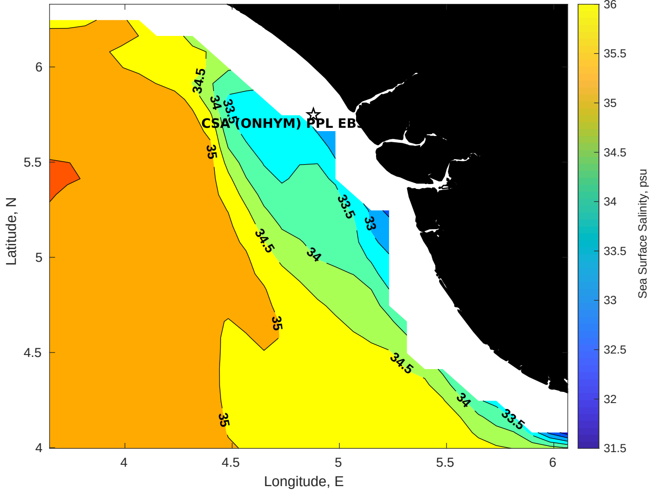
Surface Salinity for CSA (ONHYM) PPL EBS - Nigeria at 26-Aug-2025 00:00:00
