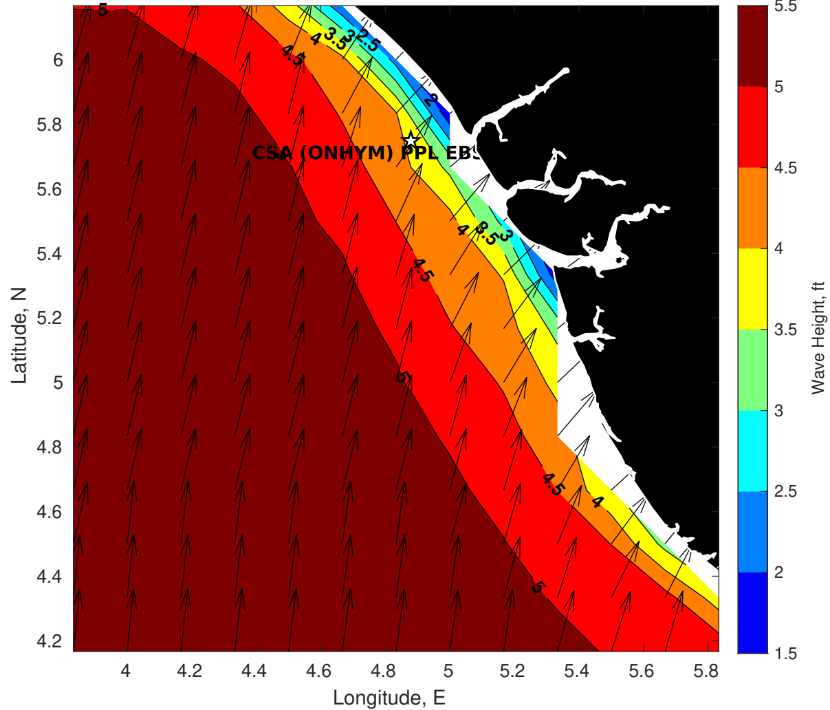
Wave Height (ft) for CSA (ONHYM) PPL EBS - Nigeria at 27-Aug-2025 09:00:00
