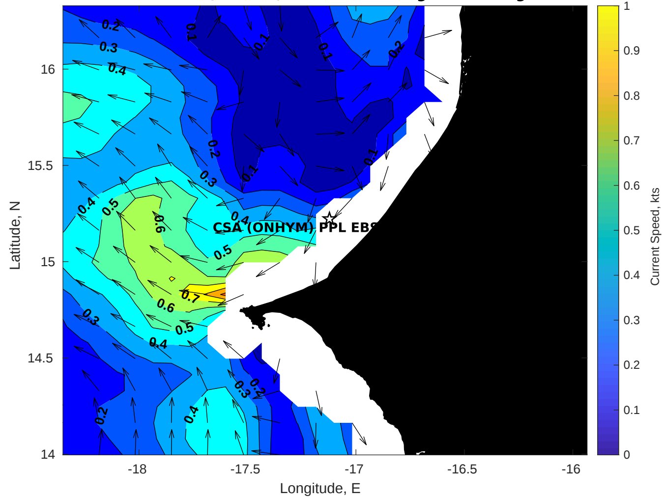
Surface Currents for CSA (ONHYM) PPL EBS - Senegal at 26-Aug-2025 00:00:00
