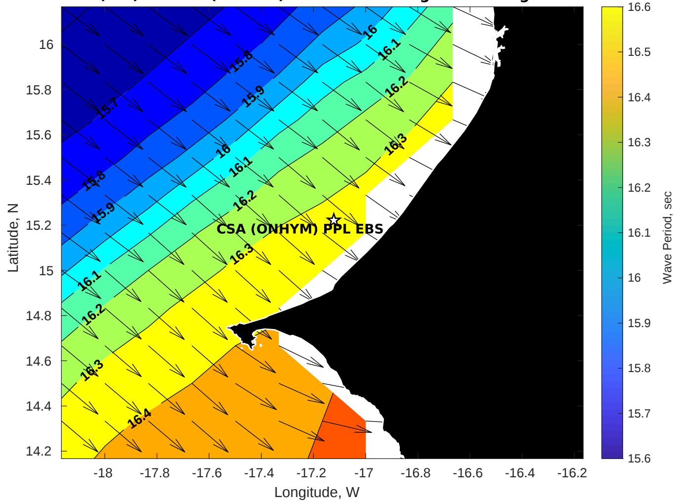
Wave Period (sec) for CSA (ONHYM) PPL EBS - Senegal at 27-Aug-2025 09:00:00
