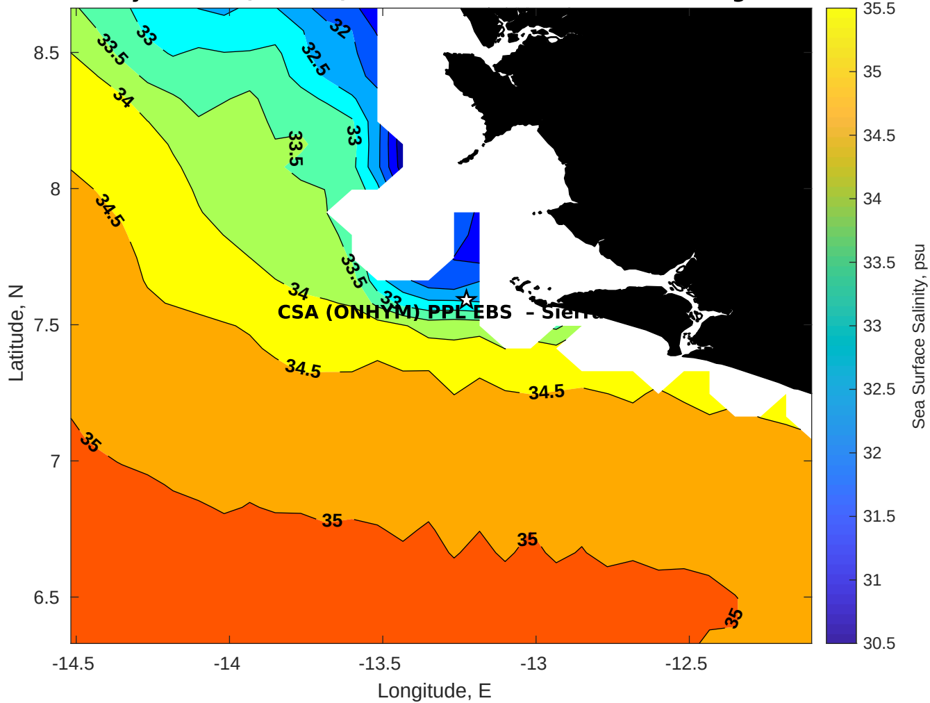
Surface Salinity for CSA (ONHYM) PPL EBS - Sierra Leone at 26-Aug-2025 00:00:00
