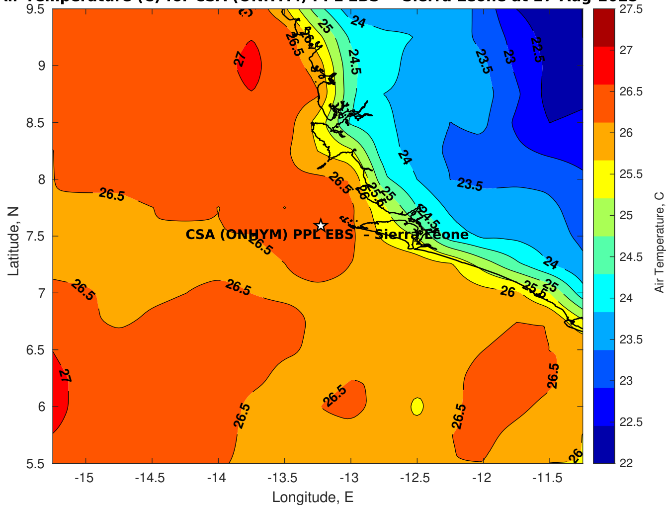
Air Temperature (C) for CSA (ONHYM) PPL EBS - Sierra Leone at 27-Aug-2025
