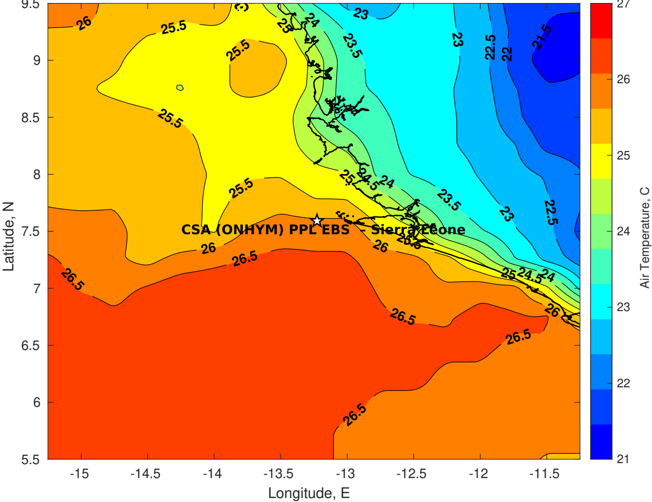
Air Temperature (C) for CSA (ONHYM) PPL EBS - Sierra Leone at 27-Aug-2025
