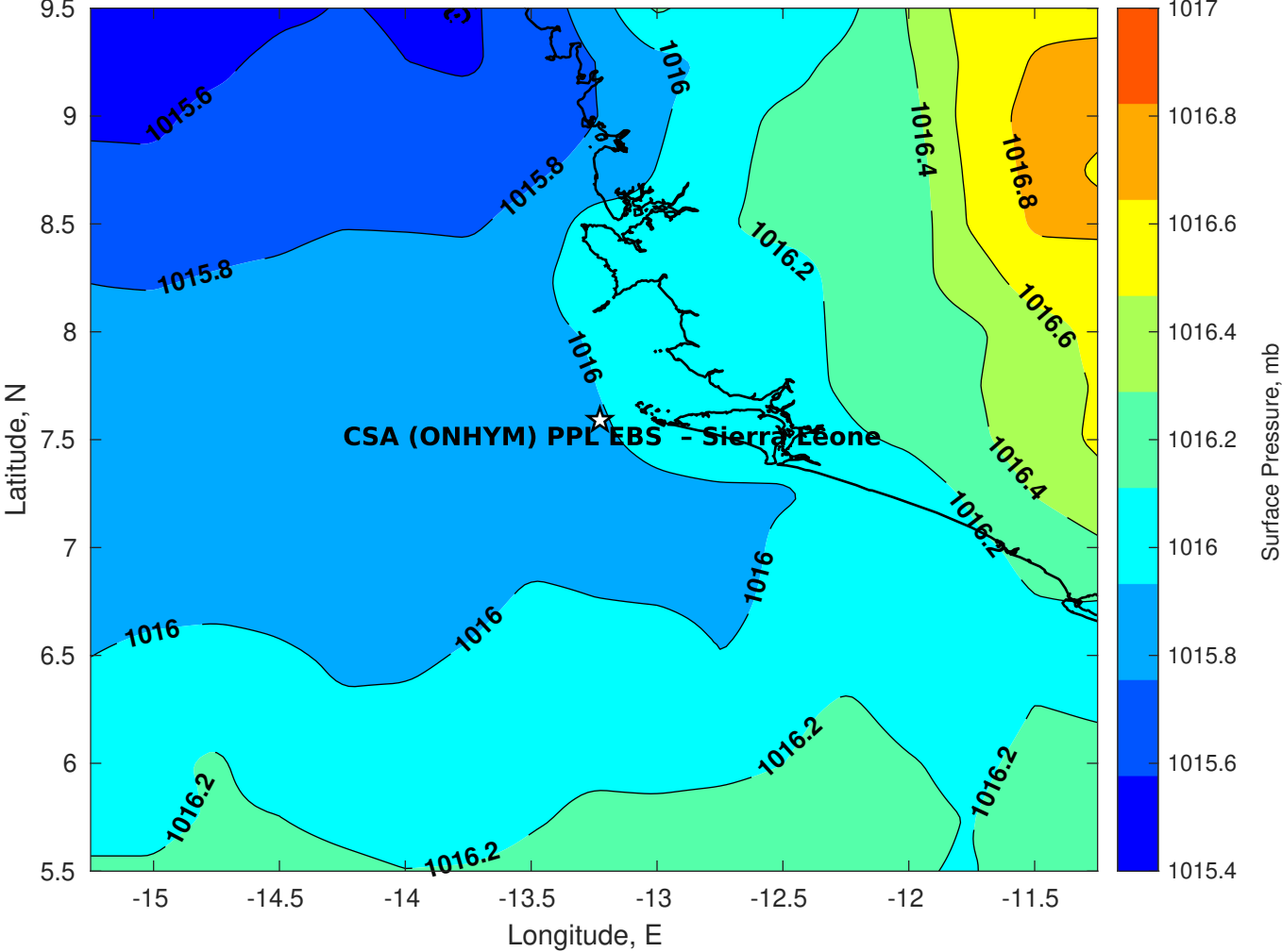
Surface Pressure (mb) for CSA (ONHYM) PPL EBS - Sierra Leone at 29-Aug-2025 00:00:00
