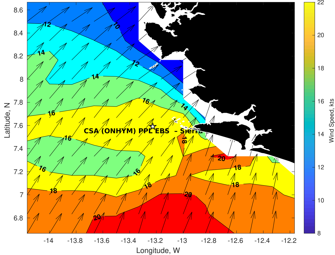
Winds (kts) for CSA (ONHYM) PPL EBS - Sierra Leone at 27-Aug-2025 09:00:00
