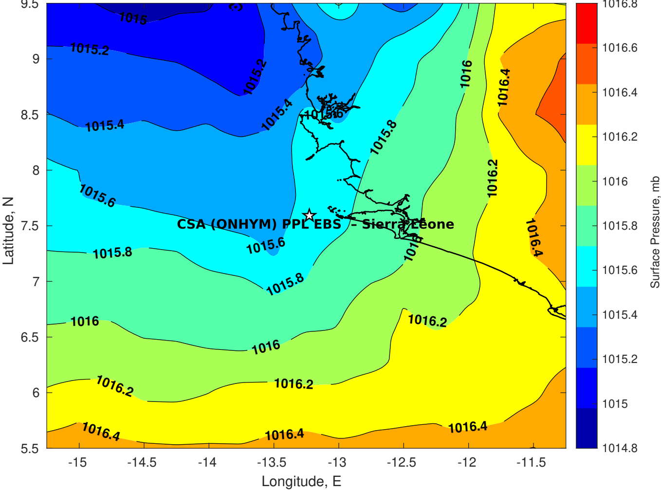
Surface Pressure (mb) for CSA (ONHYM) PPL EBS - Sierra Leone at 27-Aug-2025 00:00:00
