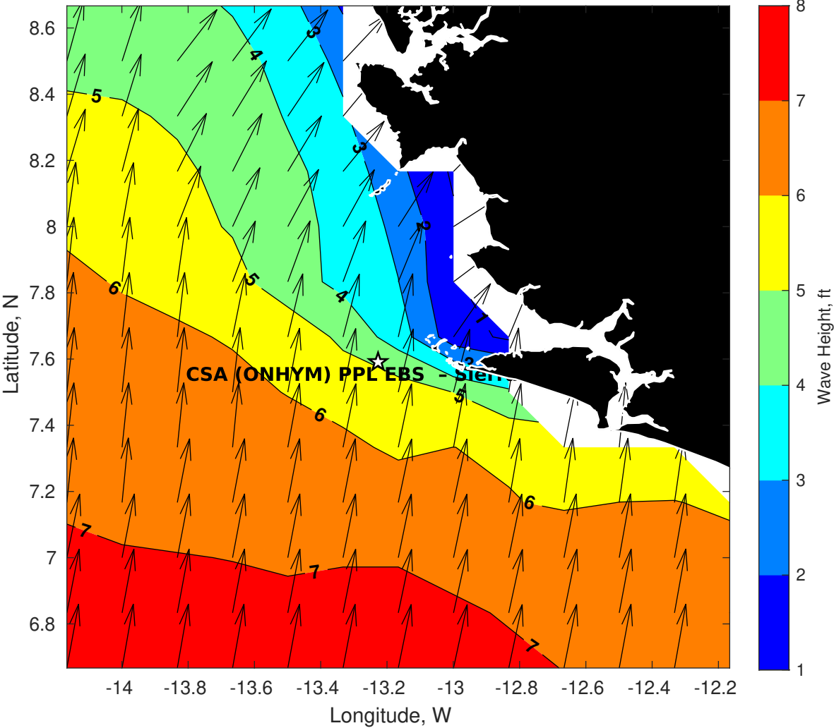
Wave Height (ft) for CSA (ONHYM) PPL EBS - Sierra Leone at 27-Aug-2025 09:00:00
