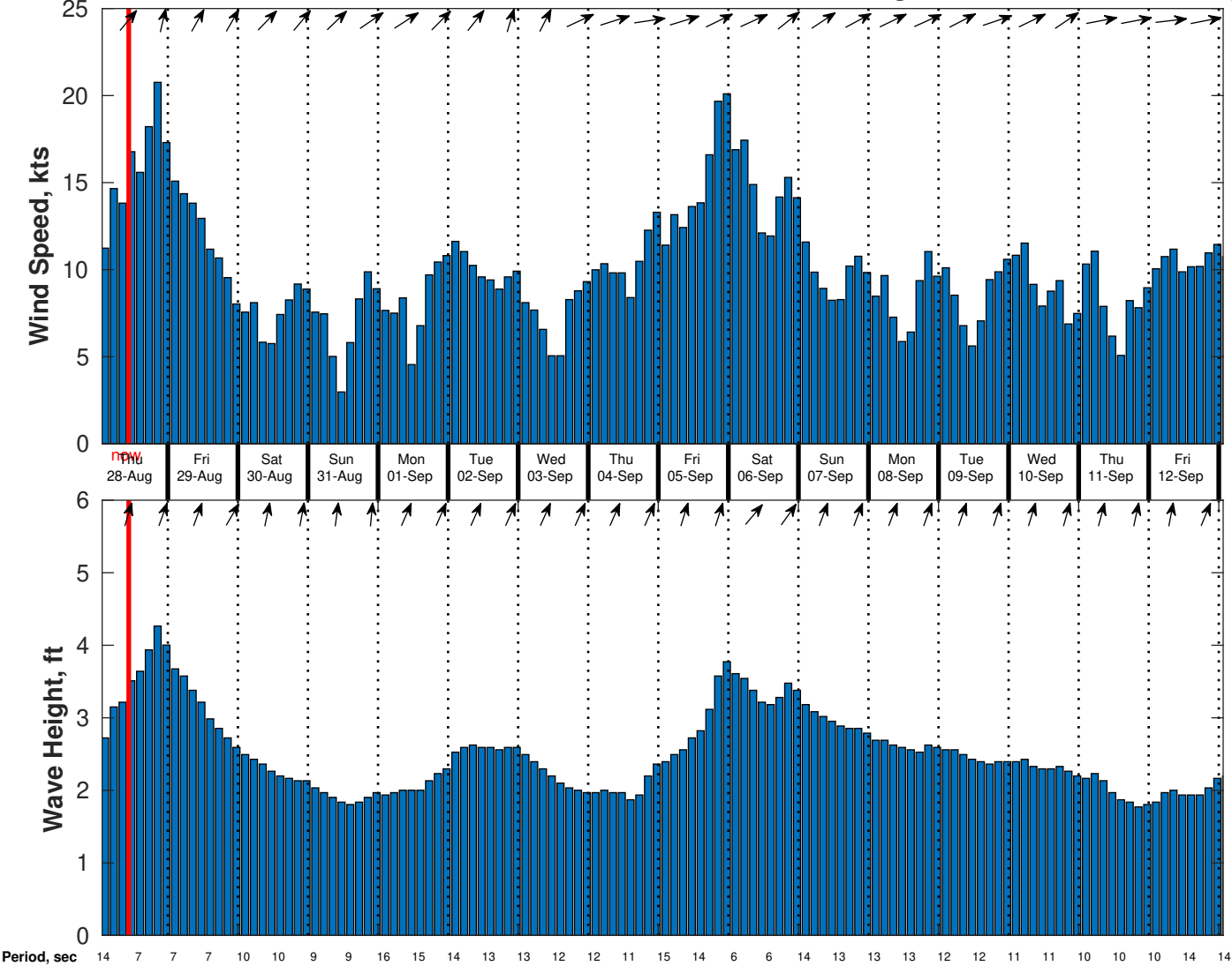
Wind & Wave Forecast for CSA (ONHYM) PPL EBS - Sierra Leone from 27-Aug-2025 01:00:00 to 12-Sep-2025 01:00:00
