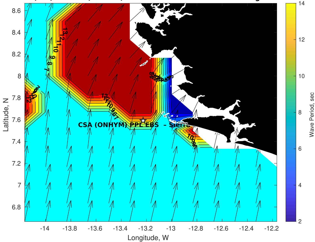
Wave Period (sec) for CSA (ONHYM) PPL EBS - Sierra Leone at 27-Aug-2025 09:00:00
