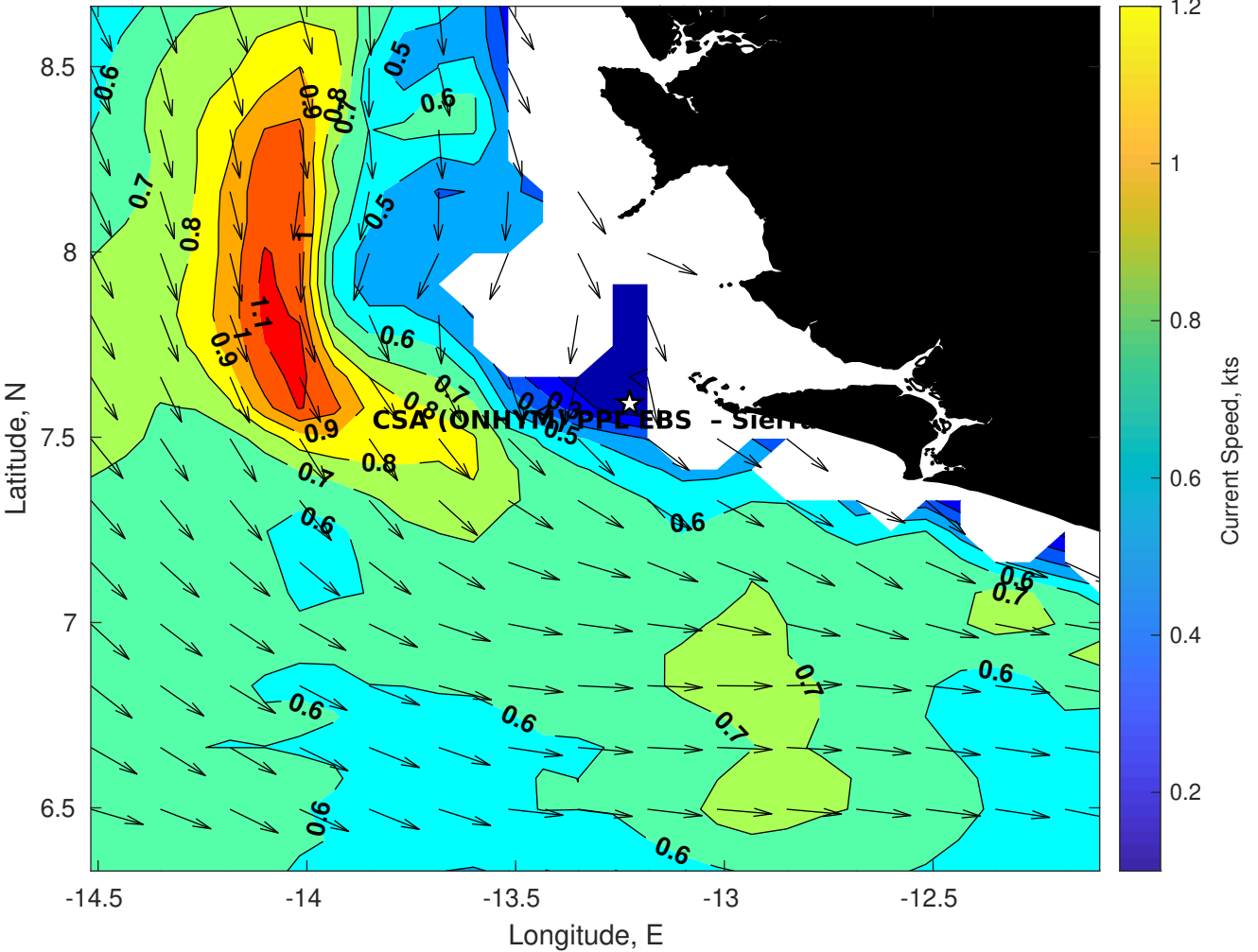
Surface Currents for CSA (ONHYM) PPL EBS - Sierra Leone at 26-Aug-2025 00:00:00
