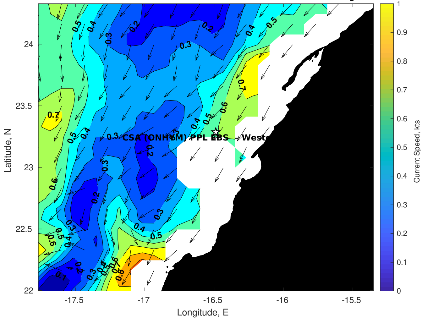
Surface Currents for CSA (ONHYM) PPL EBS - Western Sahara at 26-Aug-2025 00:00:00
