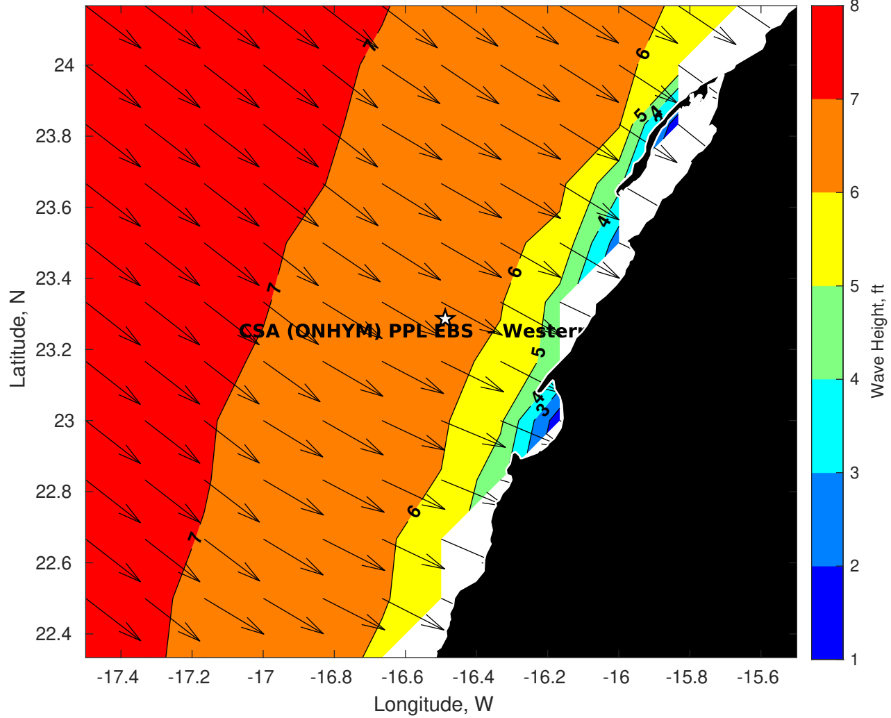
Wave Height (ft) for CSA (ONHYM) PPL EBS - Western Sahara at 27-Aug-2025 09:00:00
