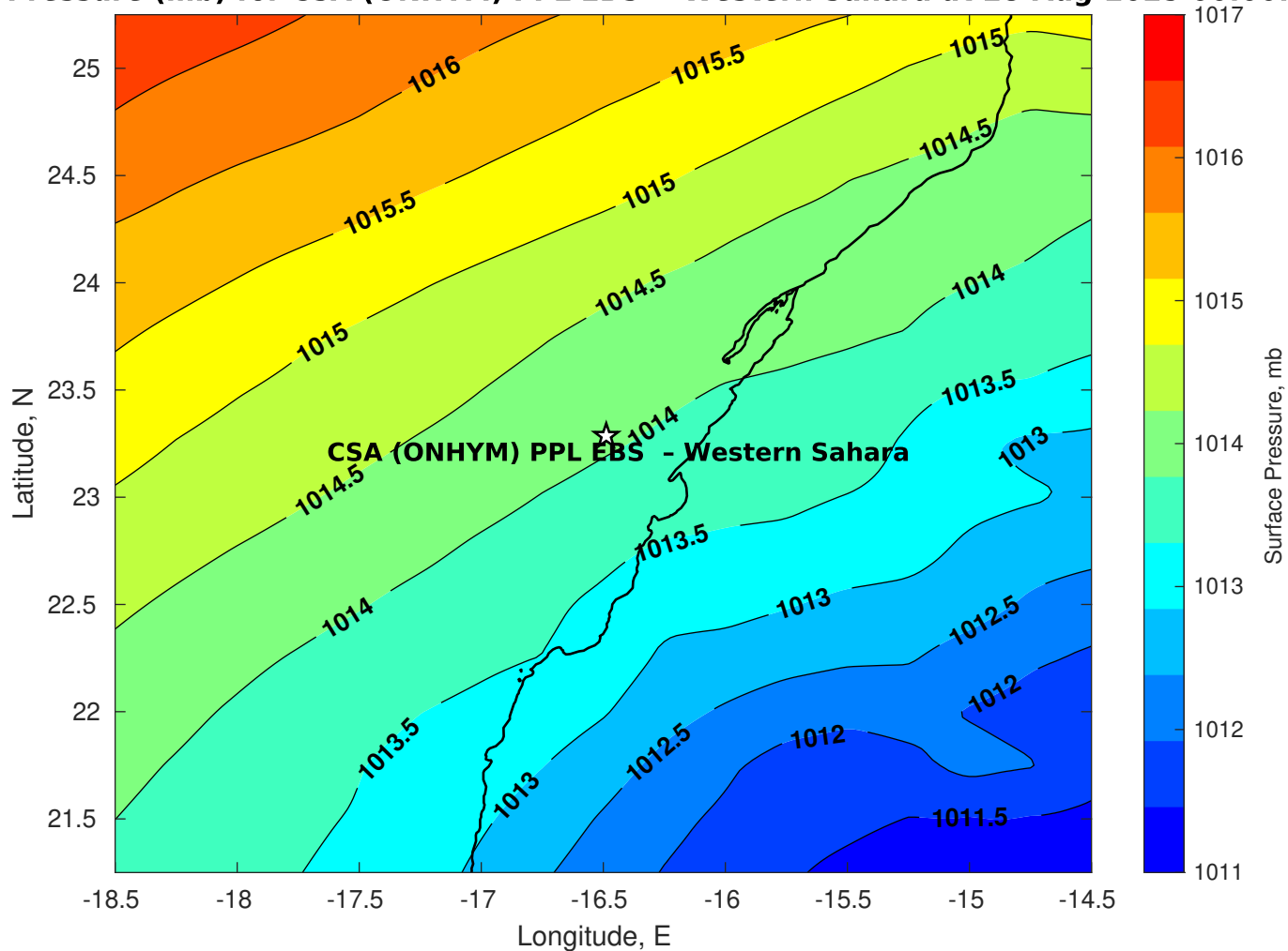
Surface Pressure (mb) for CSA (ONHYM) PPL EBS - Western Sahara at 28-Aug-2025 00:00:00
