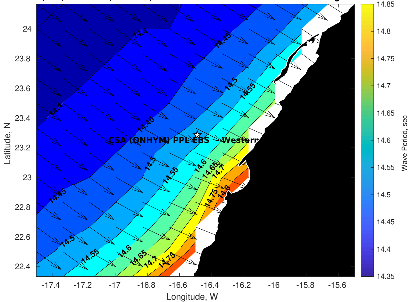
Wave Period (sec) for CSA (ONHYM) PPL EBS - Western Sahara at 27-Aug-2025 09:00:00
