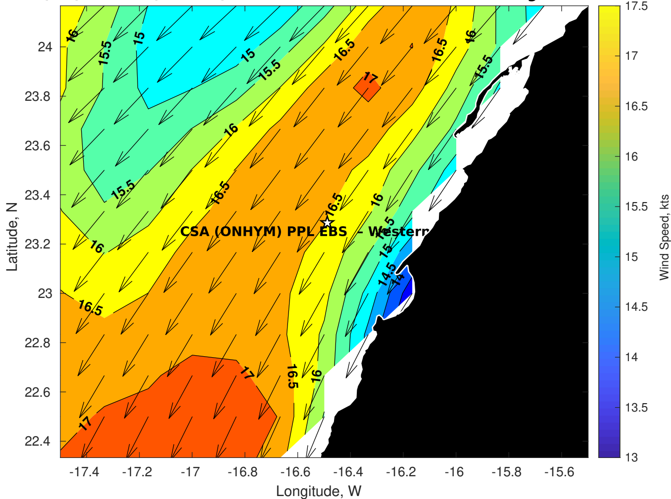
Winds (kts) for CSA (ONHYM) PPL EBS - Western Sahara at 27-Aug-2025 09:00:00
