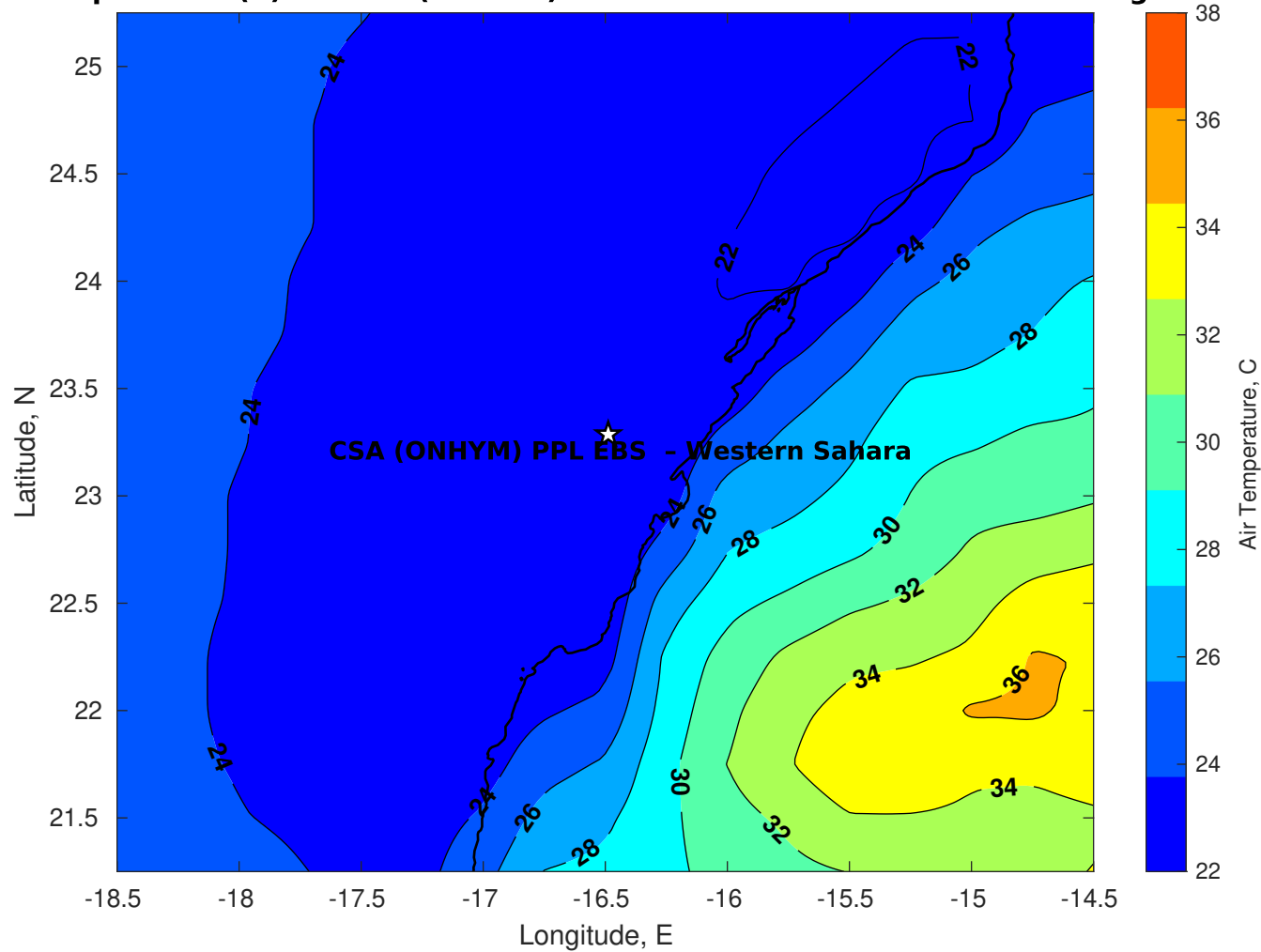
Air Temperature (C) for CSA (ONHYM) PPL EBS - Western Sahara at 27-Aug-2025
