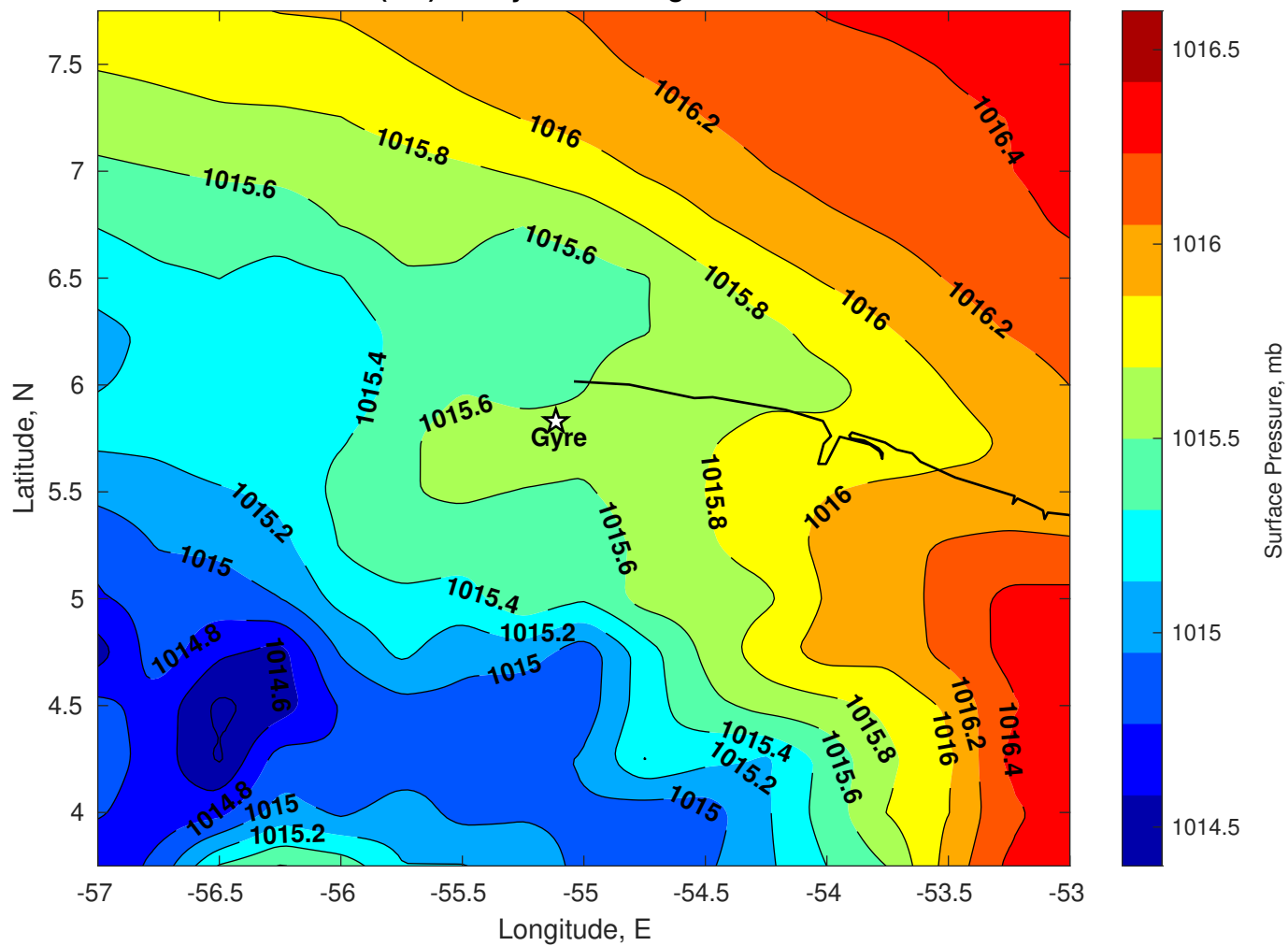
Surface Pressure (mb) for Gyre at 28-Aug-2025 00:00:00
