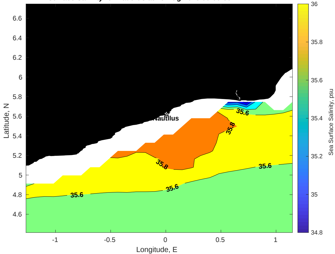
Surface Salinity for Nautilus at 26-Aug-2025 00:00:00
