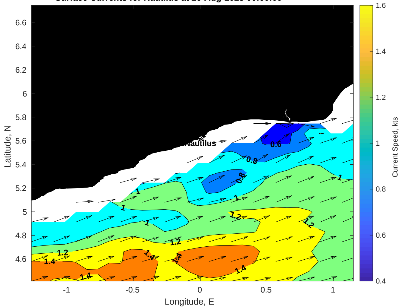
Surface Currents for Nautilus at 26-Aug-2025 00:00:00
