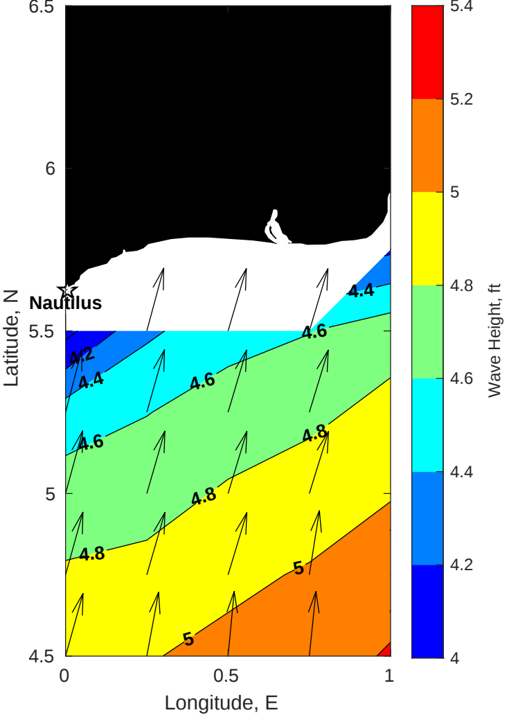
Wave Height (ft) for Nautilus at 27-Aug-2025 09:00:00
