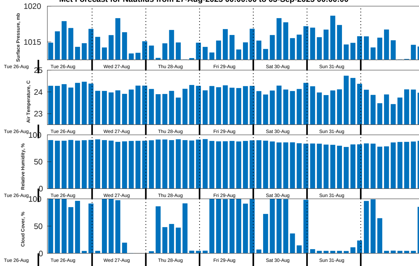
Met Forecast for Nautilus from 27-Aug-2025 00:00:00 to 03-Sep-2025 00:00:00
