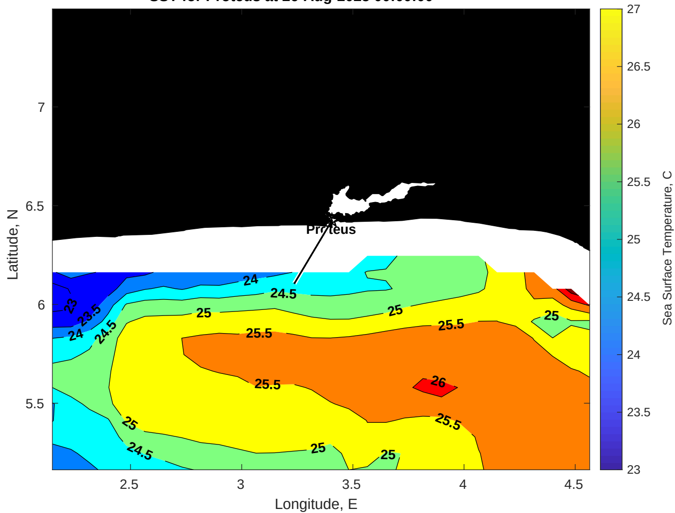
SST for Proteus at 26-Aug-2025 00:00:00
