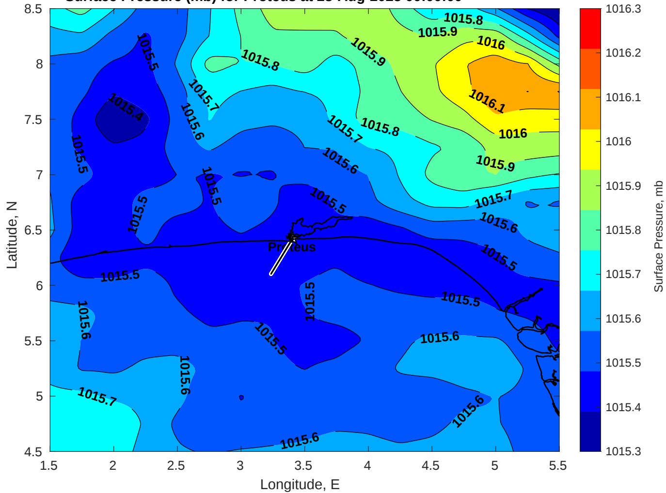
Surface Pressure (mb) for Proteus at 28-Aug-2025 00:00:00
