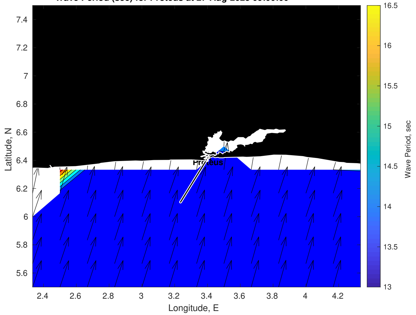
Wave Period (sec) for Proteus at 27-Aug-2025 09:00:00
