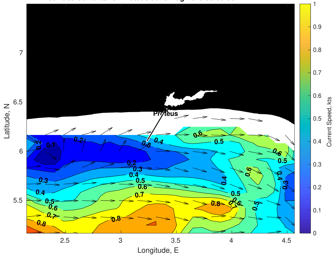
Surface Currents for Proteus at 26-Aug-2025 00:00:00
