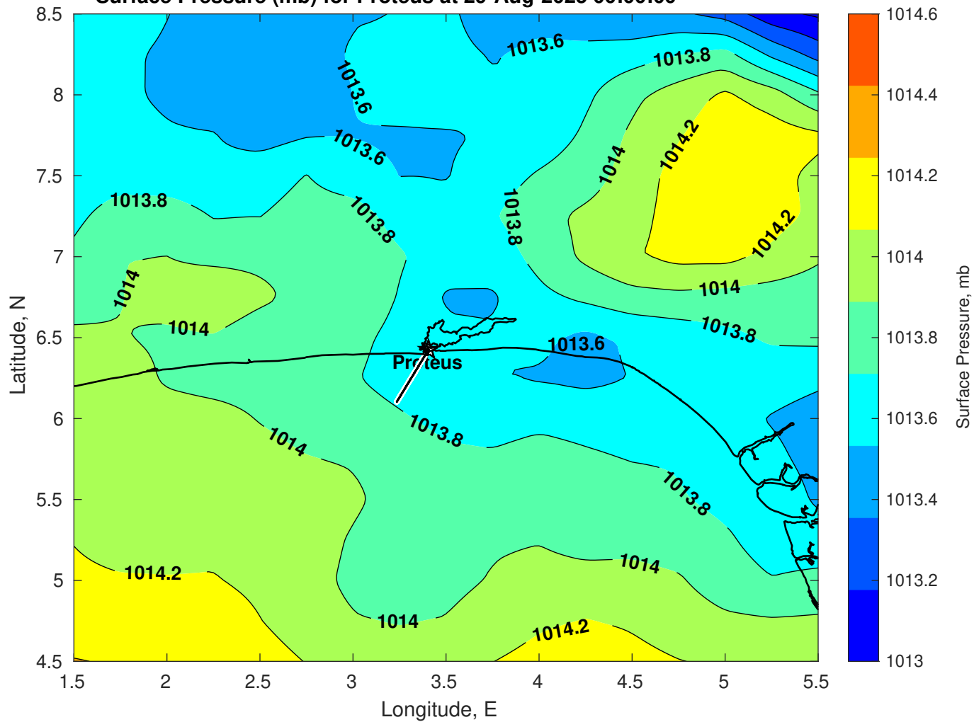
Surface Pressure (mb) for Proteus at 29-Aug-2025 00:00:00
