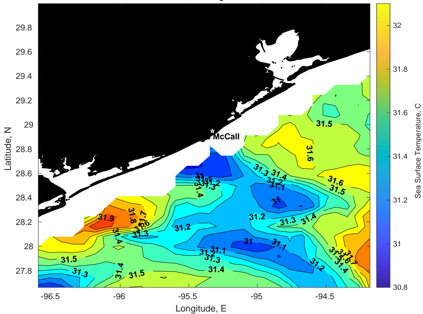
SST for Brooks McCall at 27-Aug-2025 00:00:00
