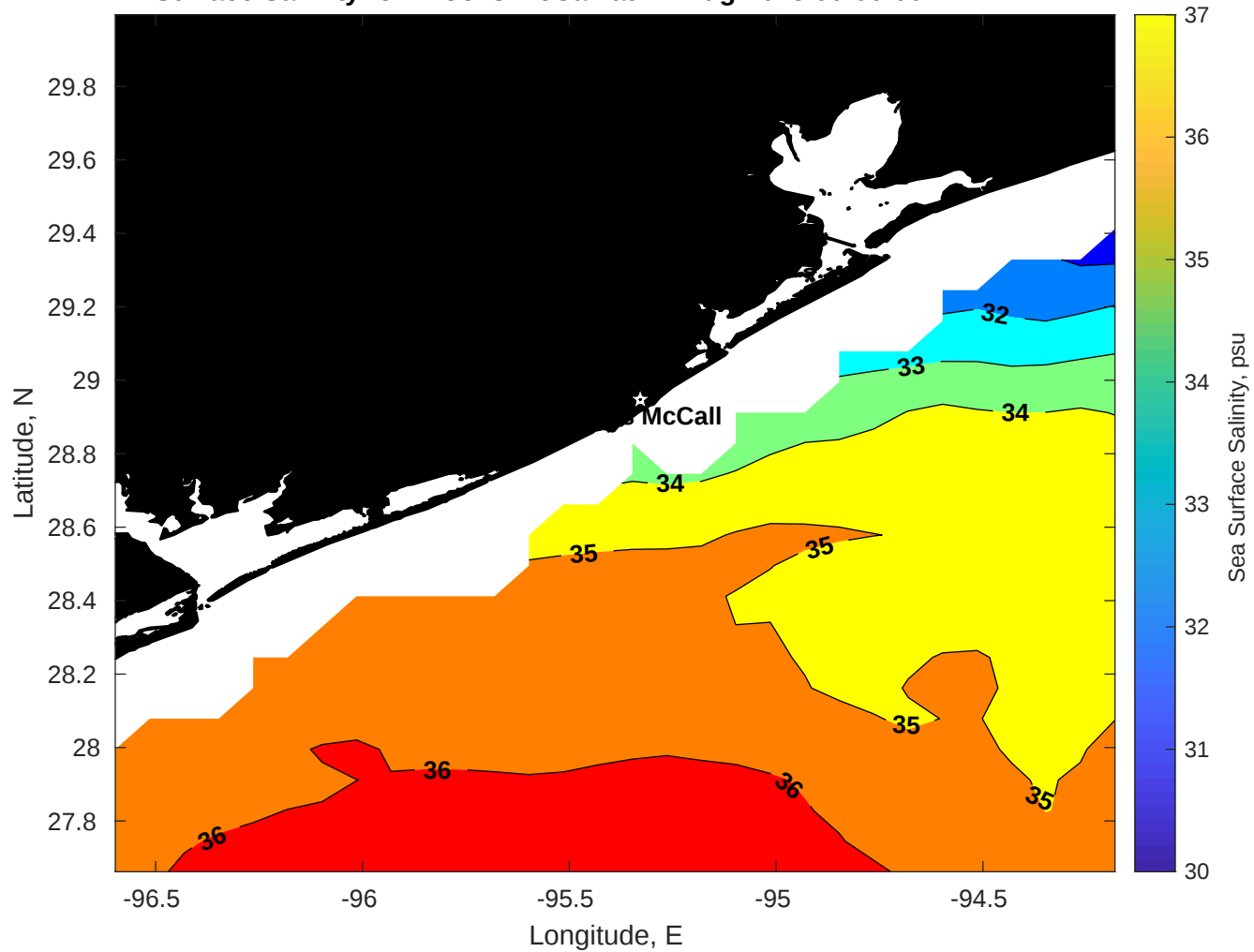
Surface Salinity for Brooks McCall at 27-Aug-2025 00:00:00
