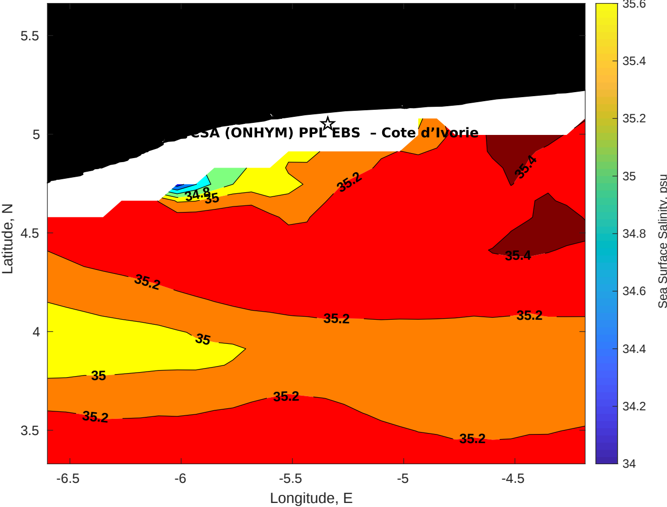
Surface Salinity for CSA (ONHYM) PPL EBS - Cote d'Ivoire at 27-Aug-2025 00:00:00
