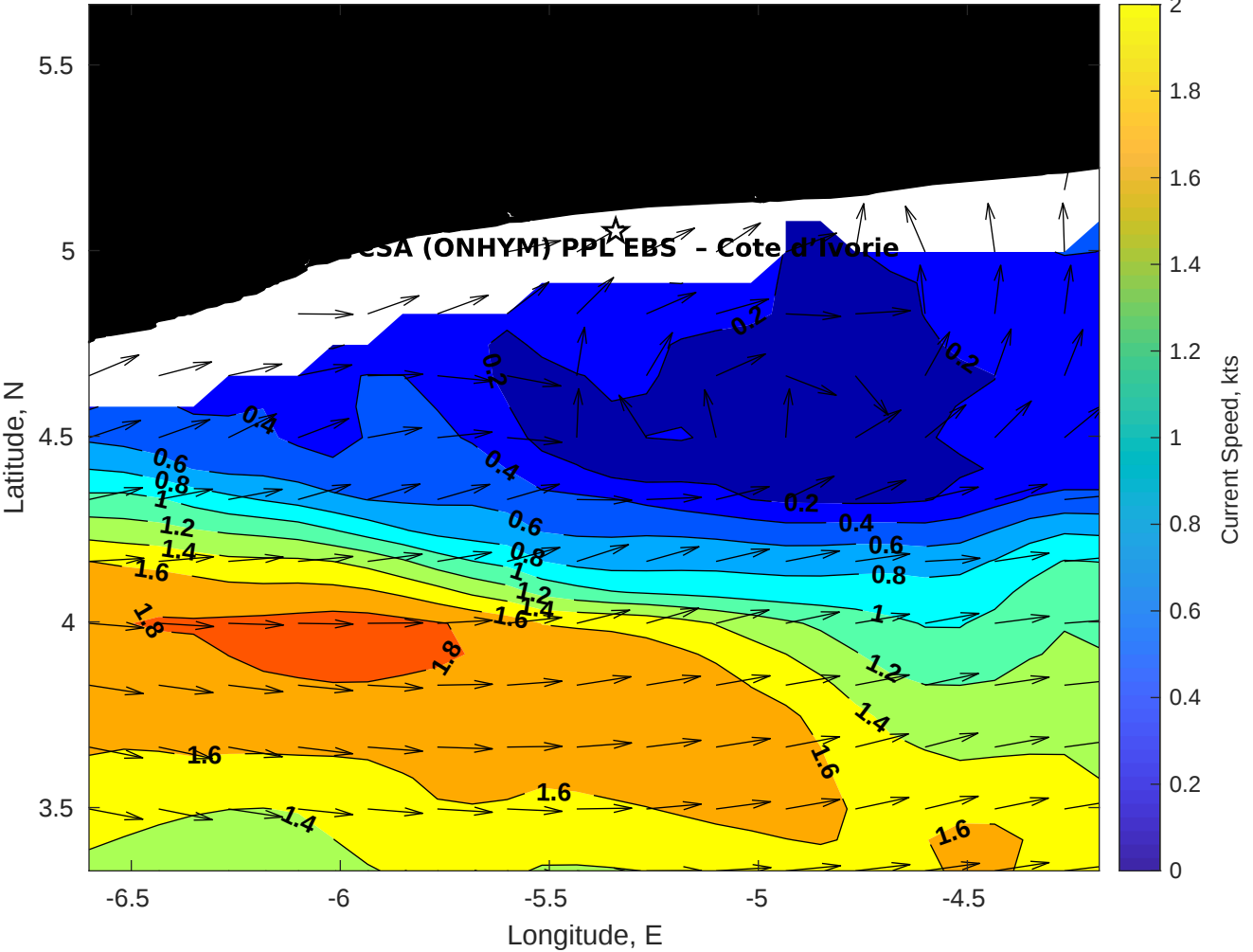
Surface Currents for CSA (ONHYM) PPL EBS - Cote d'Ivoire at 27-Aug-2025 00:00:00
