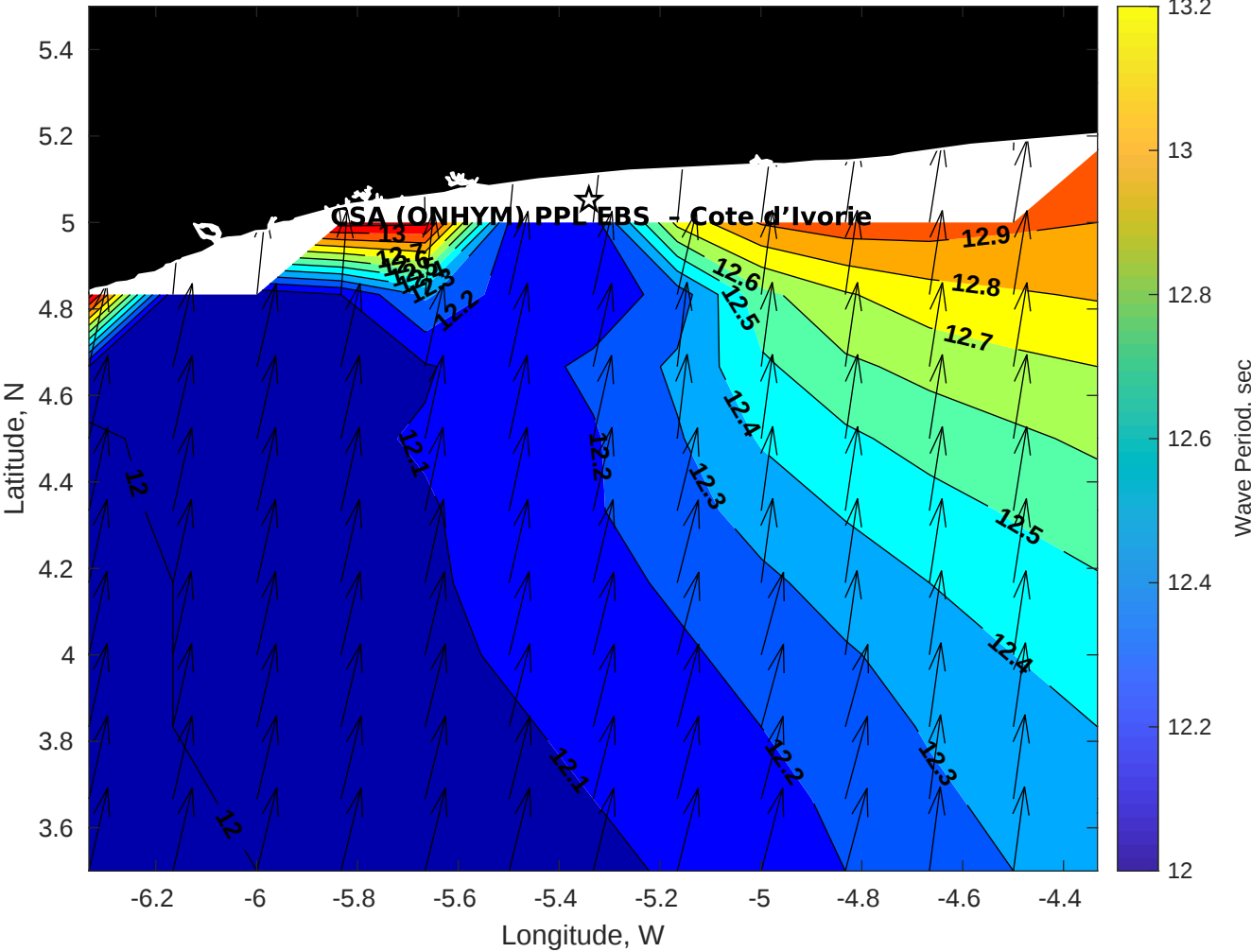
Wave Period (sec) for CSA (ONHYM) PPL EBS - Cote d'Ivoire at 28-Aug-2025 09:00:00
