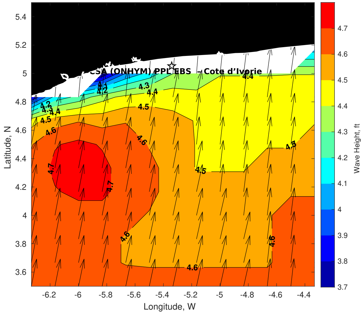
Wave Height (ft) for CSA (ONHYM) PPL EBS - Cote d'Ivoire at 28-Aug-2025 09:00:00
