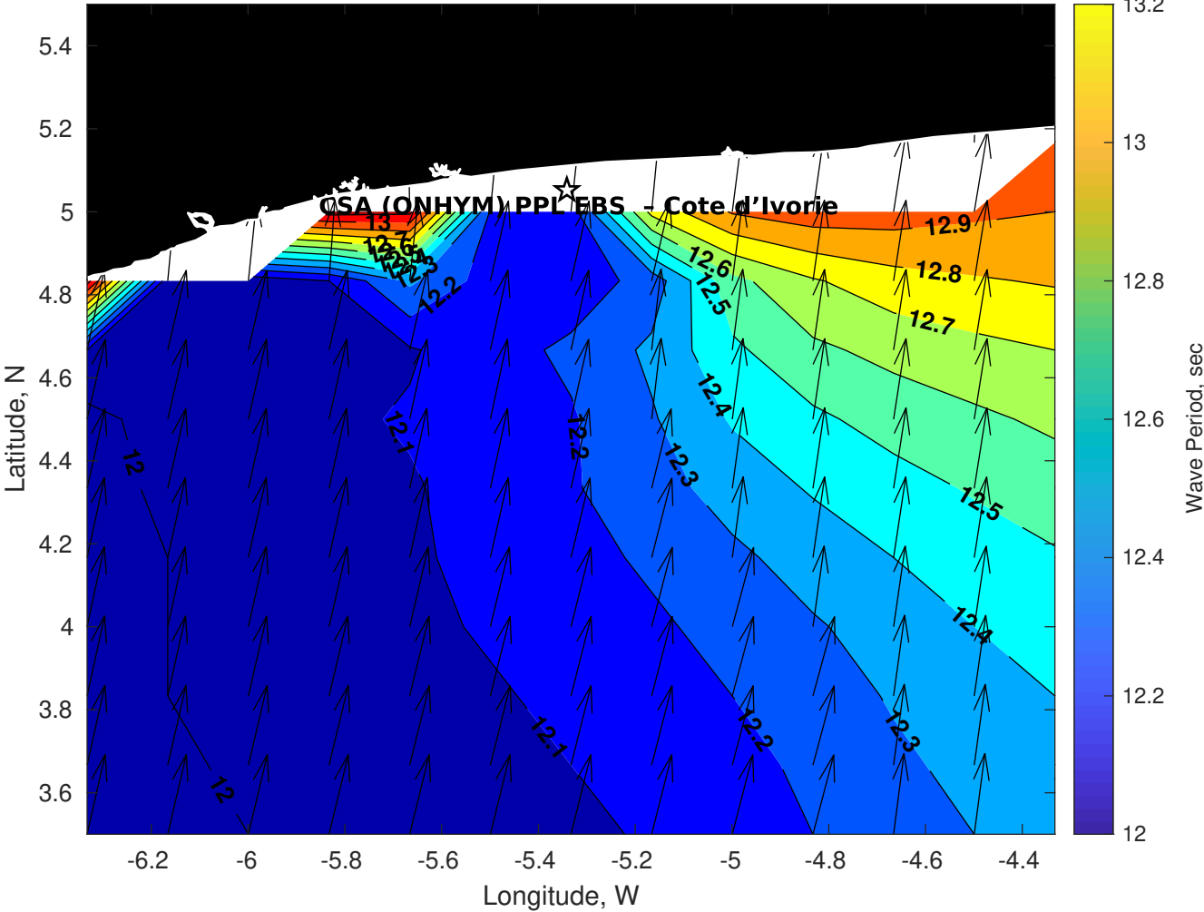
Wave Period (sec) for CSA (ONHYM) PPL EBS - Cote d'Ivoire at 28-Aug-2025 09:00:00
