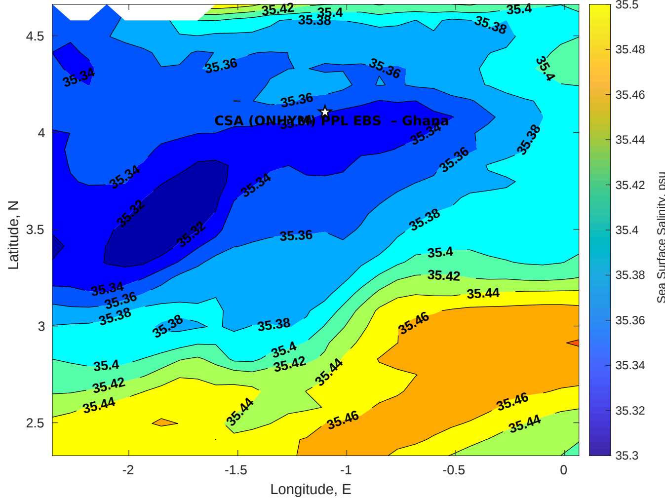
Surface Salinity for CSA (ONHYM) PPL EBS - Ghana at 27-Aug-2025 00:00:00
