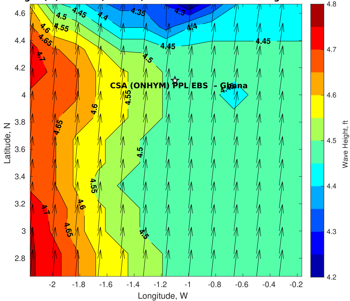
Wave Height (ft) for CSA (ONHYM) PPL EBS - Ghana at 28-Aug-2025 09:00:00
