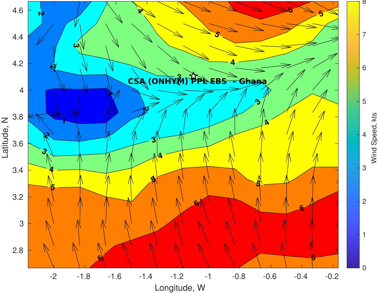
Winds (kts) for CSA (ONHYM) PPL EBS - Ghana at 28-Aug-2025 09:00:00
