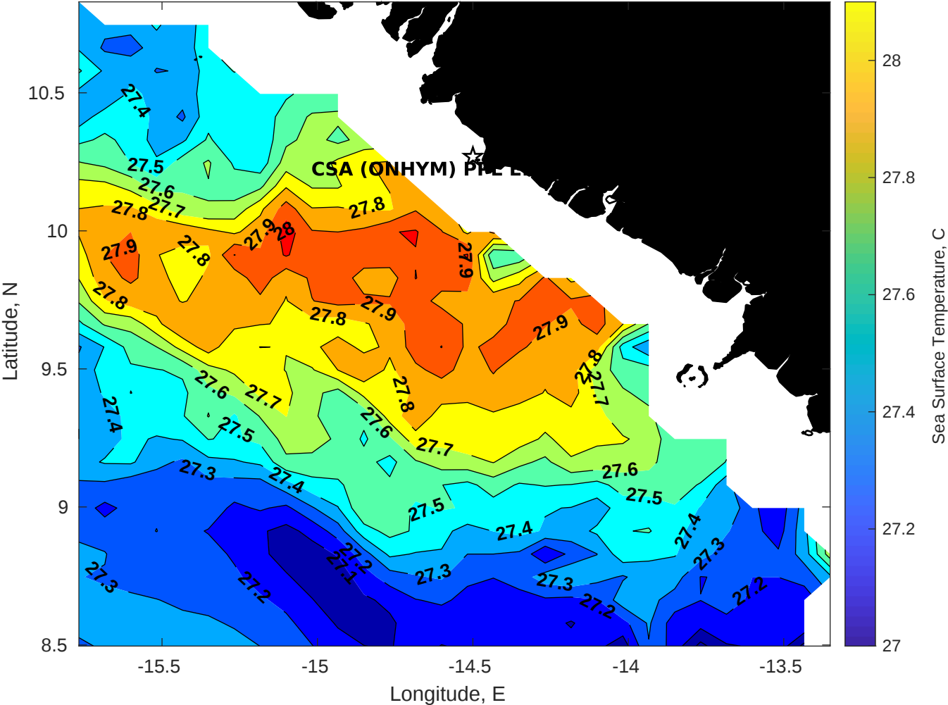
SST for CSA (ONHYM) PPL EBS - Guinea at 27-Aug-2025 00:00:00
