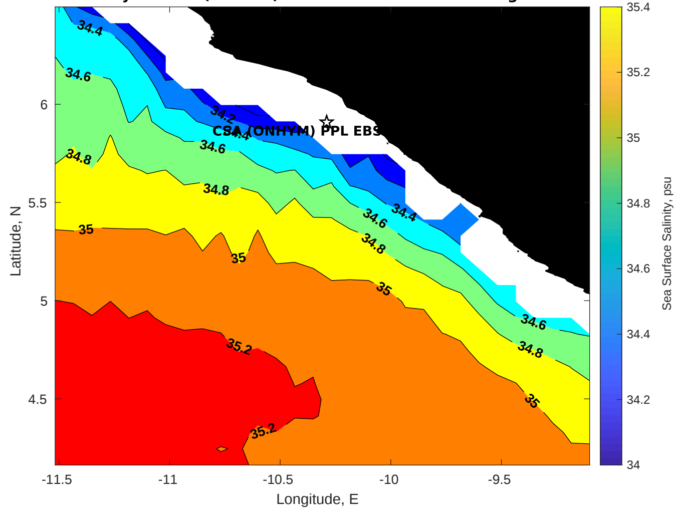
Surface Salinity for CSA (ONHYM) PPL EBS - Liberia at 27-Aug-2025 00:00:00
