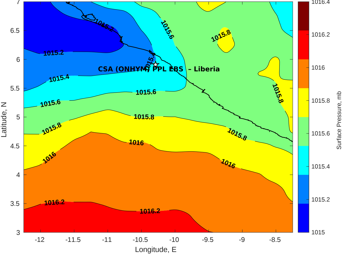
Surface Pressure (mb) for CSA (ONHYM) PPL EBS - Liberia at 30-Aug-2025 00:00:00
