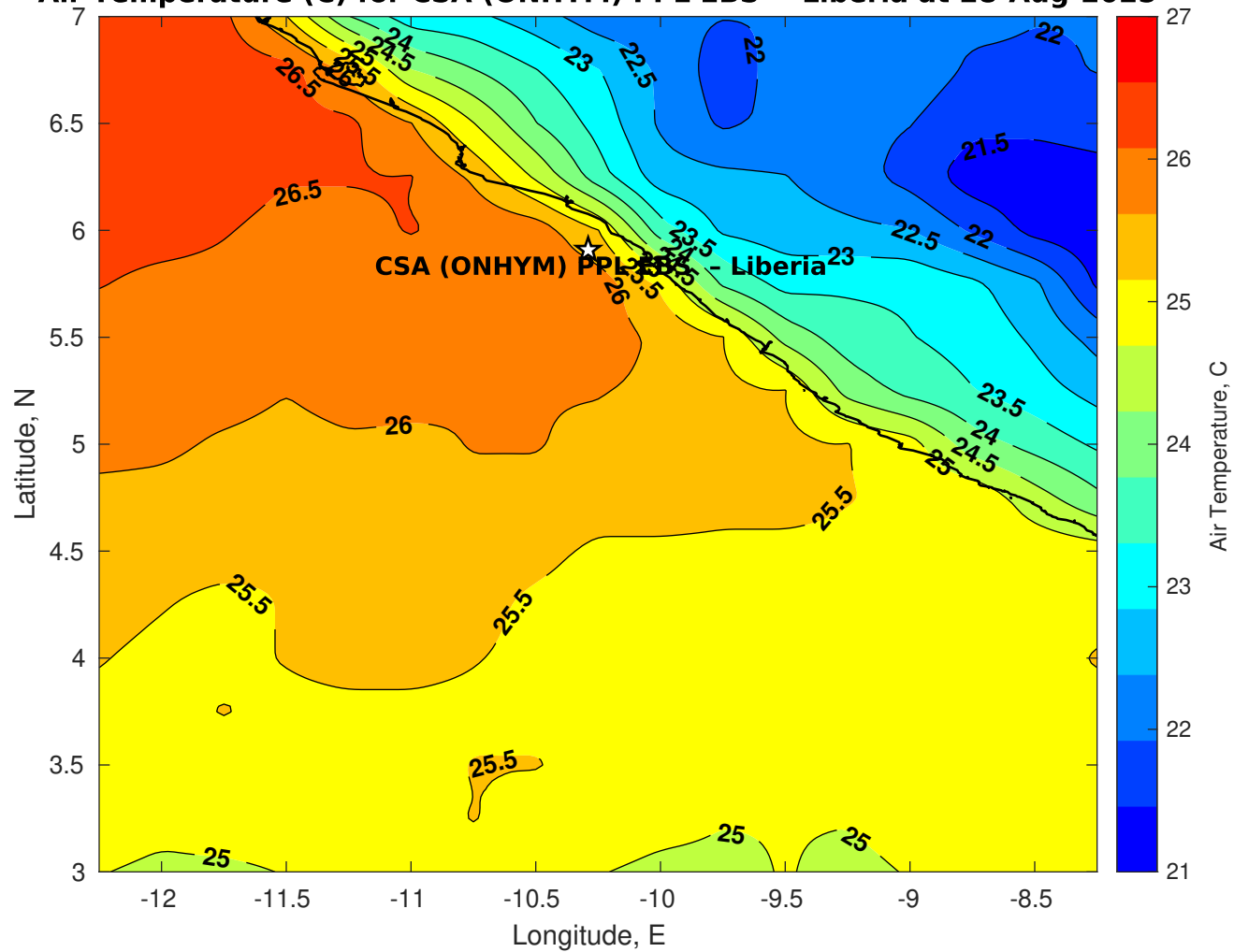
Air Temperature (C) for CSA (ONHYM) PPL EBS - Liberia at 28-Aug-2025
