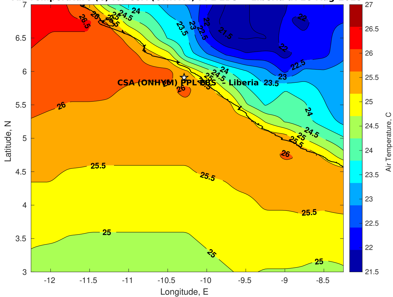
Air Temperature (C) for CSA (ONHYM) PPL EBS - Liberia at 28-Aug-2025
