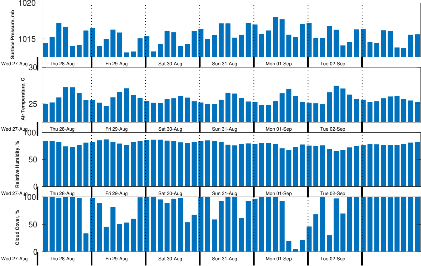
Met Forecast for CSA (ONHYM) PPL EBS - Liberia from 28-Aug-2025 00:00:00 to 04-Sep-2025 00:00:00
