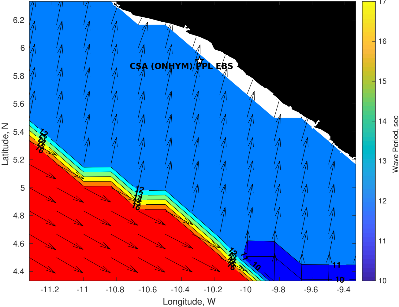
Wave Period (sec) for CSA (ONHYM) PPL EBS - Liberia at 28-Aug-2025 09:00:00
