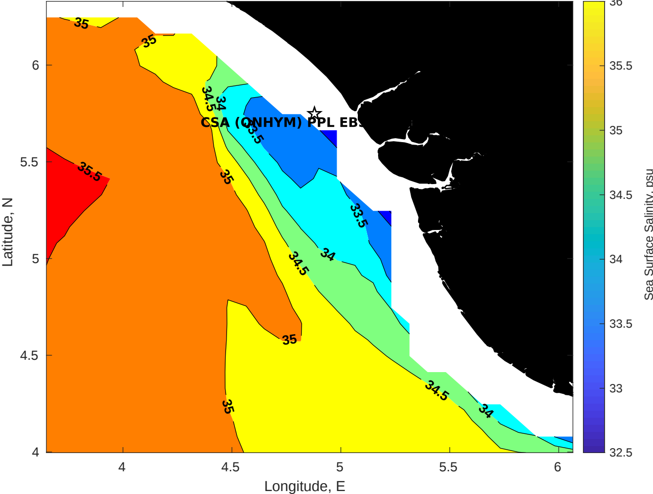
Surface Salinity for CSA (ONHYM) PPL EBS - Nigeria at 27-Aug-2025 00:00:00
