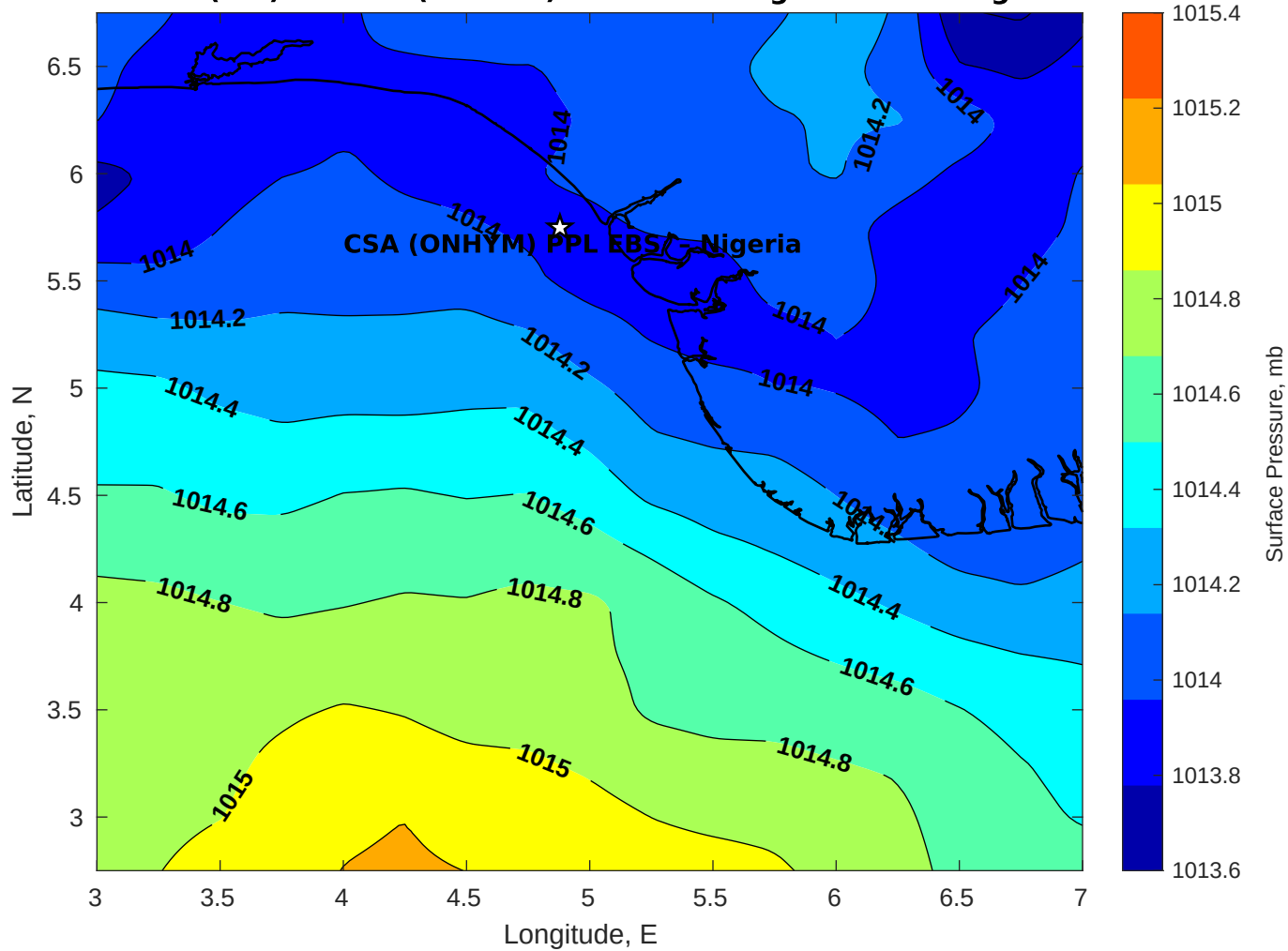
Surface Pressure (mb) for CSA (ONHYM) PPL EBS - Nigeria at 29-Aug-2025 00:00:00
