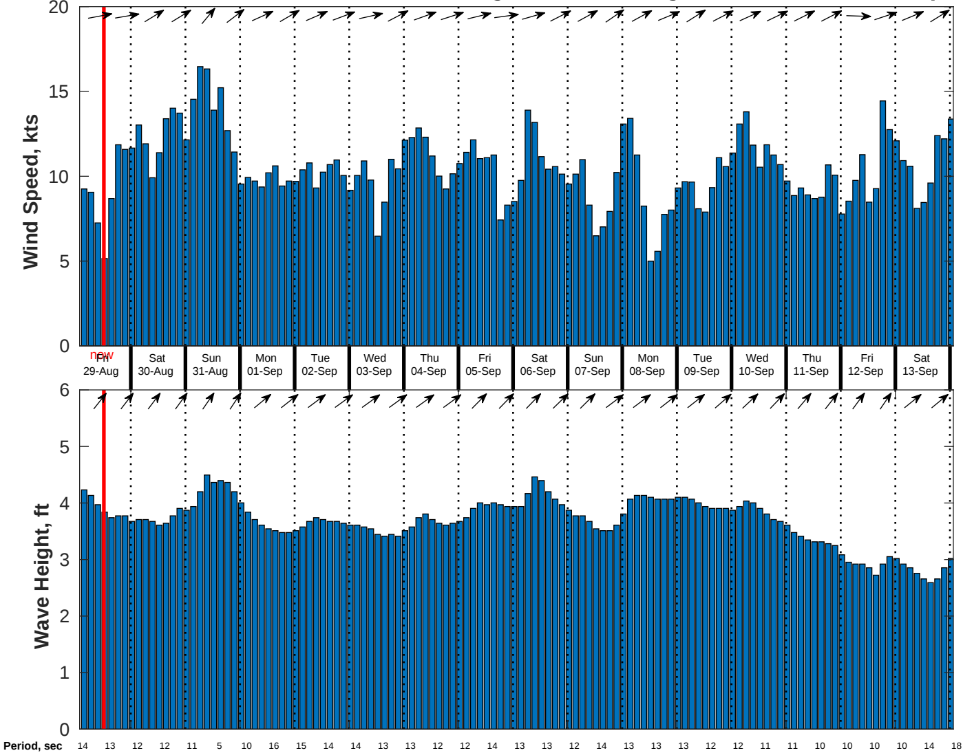
Wind & Wave Forecast for CSA (ONHYM) PPL EBS - Nigeria from 28-Aug-2025 02:00:00 to 13-Sep-2025 02:00:00
