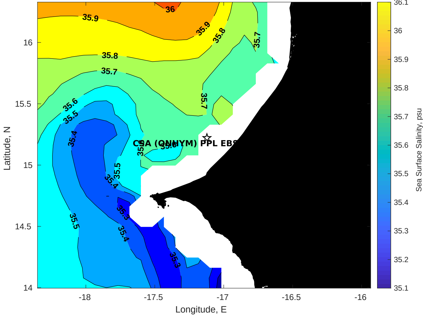
Surface Salinity for CSA (ONHYM) PPL EBS - Senegal at 27-Aug-2025 00:00:00
