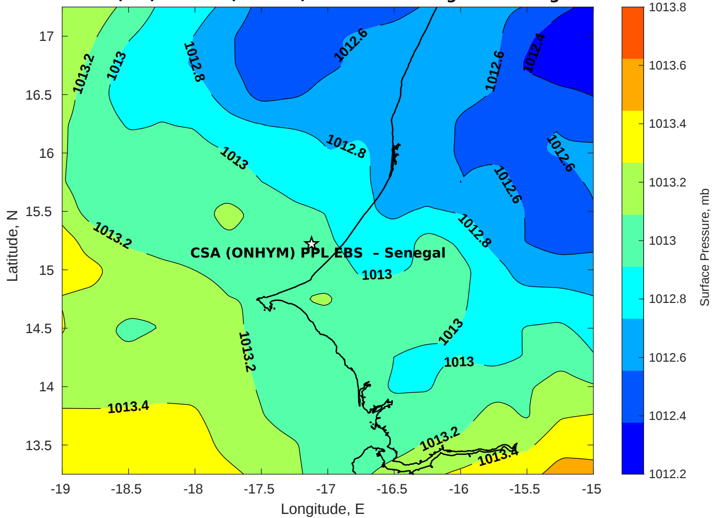
Surface Pressure (mb) for CSA (ONHYM) PPL EBS - Senegal at 28-Aug-2025 00:00:00
