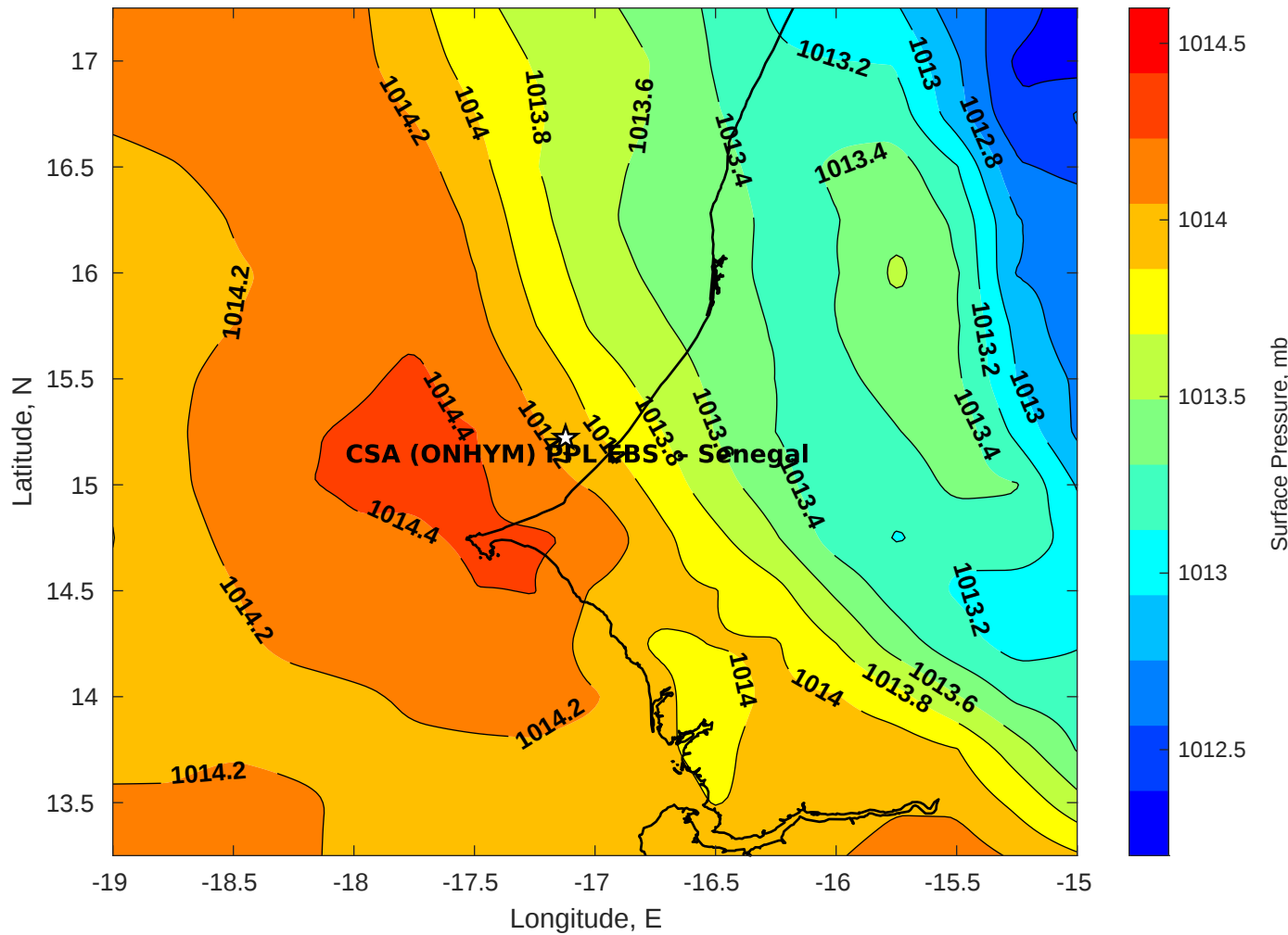
Surface Pressure (mb) for CSA (ONHYM) PPL EBS - Senegal at 30-Aug-2025 00:00:00
