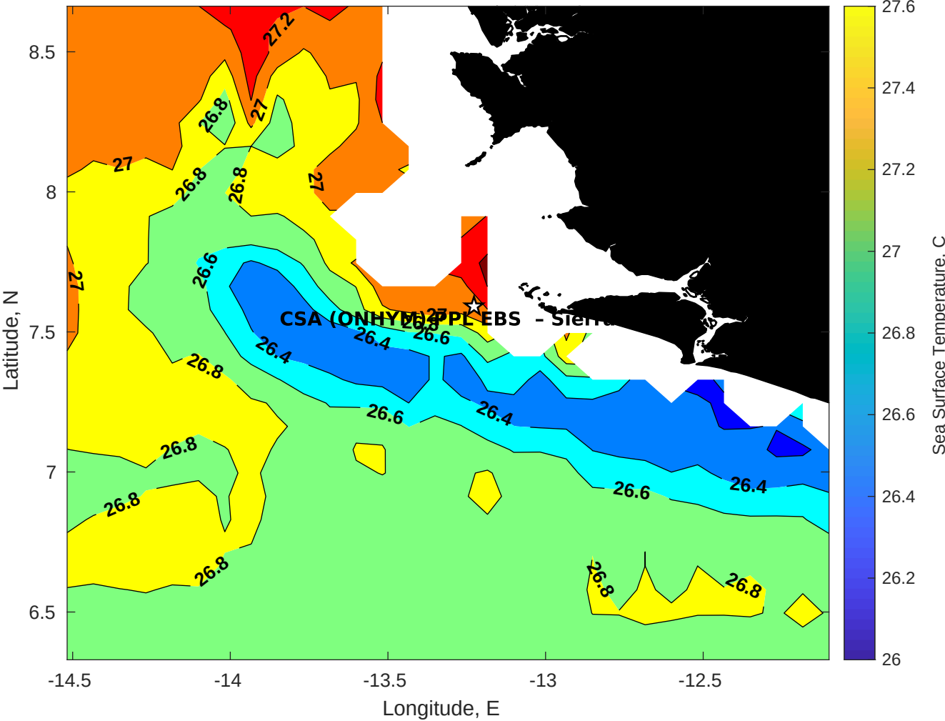
SST for CSA (ONHYM) PPL EBS - Sierra Leone at 27-Aug-2025 00:00:00
