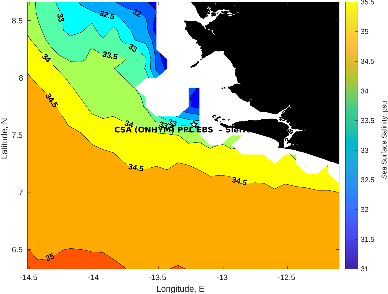
Surface Salinity for CSA (ONHYM) PPL EBS - Sierra Leone at 27-Aug-2025 00:00:00
