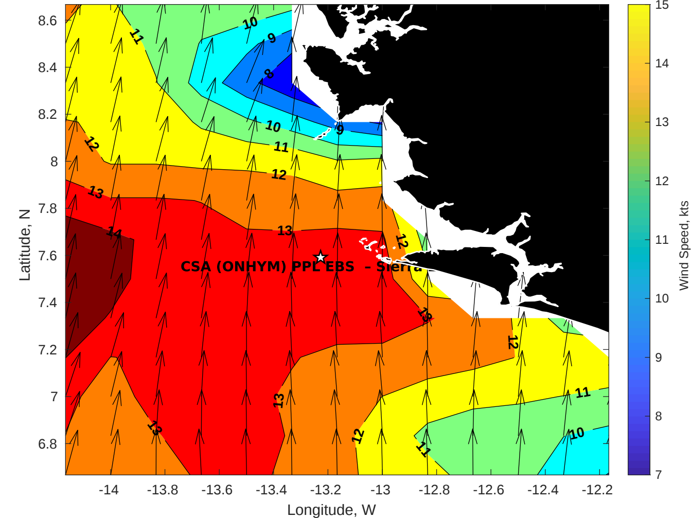
Winds (kts) for CSA (ONHYM) PPL EBS - Sierra Leone at 28-Aug-2025 09:00:00
