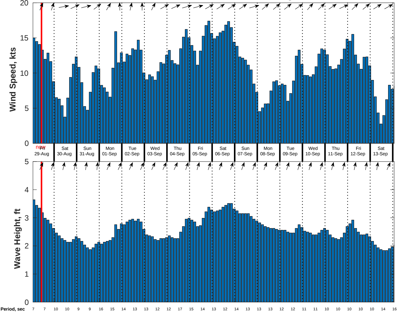
Wind & Wave Forecast for CSA (ONHYM) PPL EBS - Sierra Leone from 28-Aug-2025 01:00:00 to 13-Sep-2025 01:00:00
