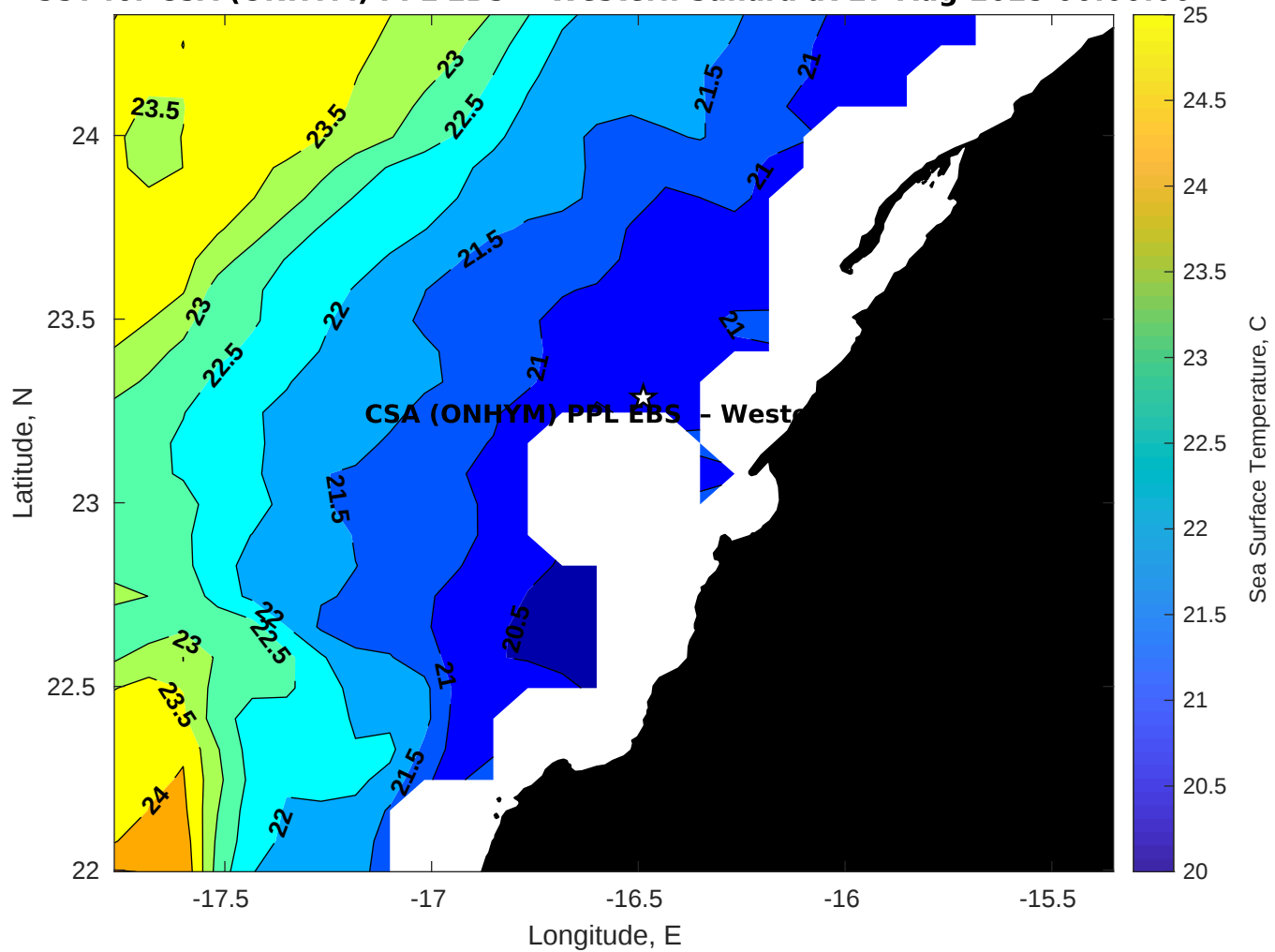
SST for CSA (ONHYM) PPL EBS - Western Sahara at 27-Aug-2025 00:00:00
