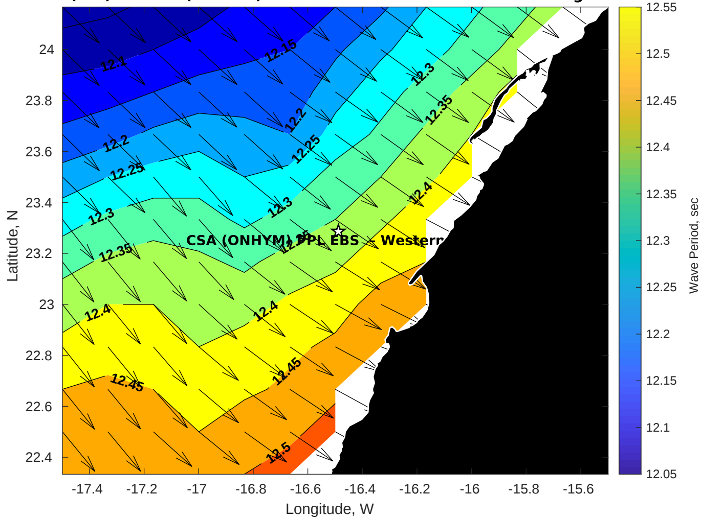
Wave Period (sec) for CSA (ONHYM) PPL EBS - Western Sahara at 28-Aug-2025 09:00:00
