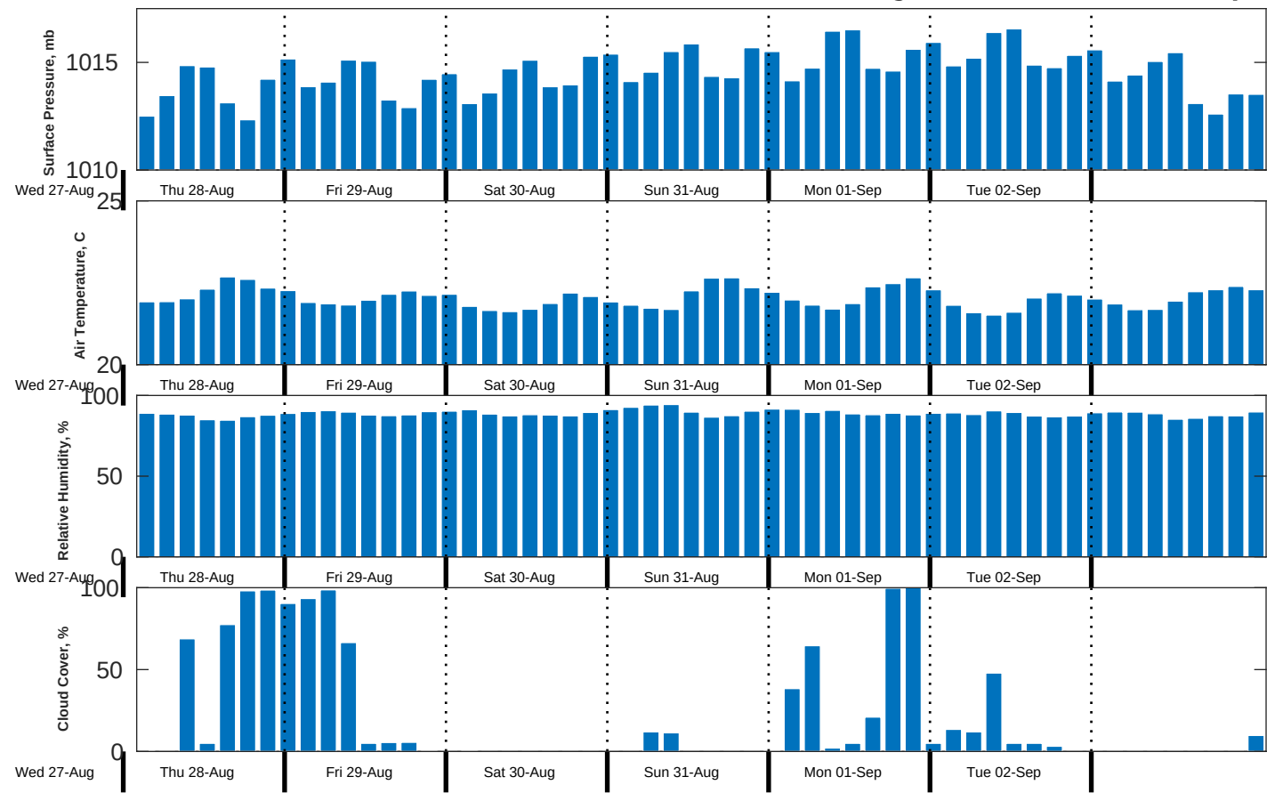
Met Forecast for CSA (ONHYM) PPL EBS - Western Sahara from 28-Aug-2025 00:00:00 to 04-Sep-2025 00:00:00
