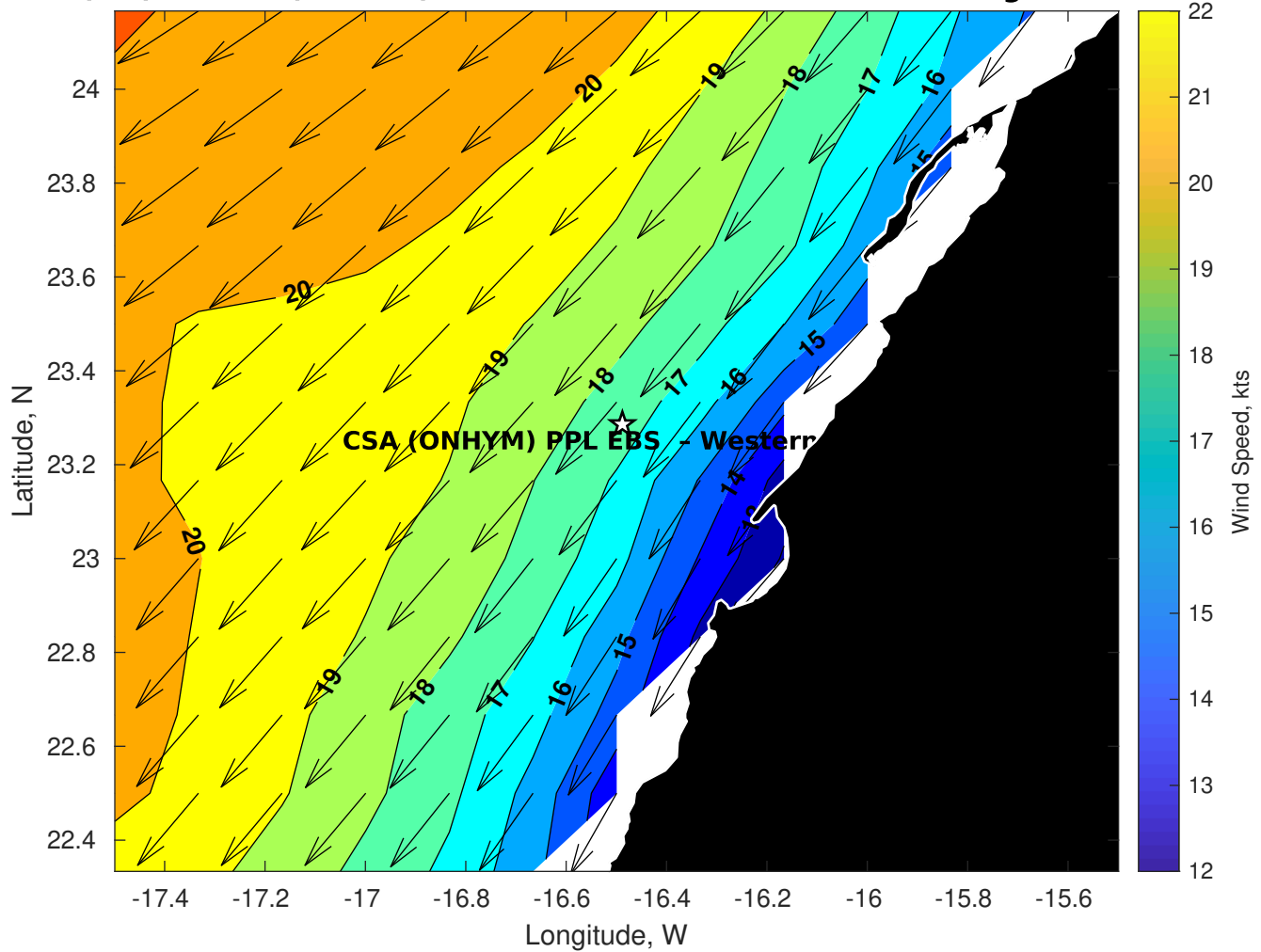
Winds (kts) for CSA (ONHYM) PPL EBS - Western Sahara at 28-Aug-2025 09:00:00
