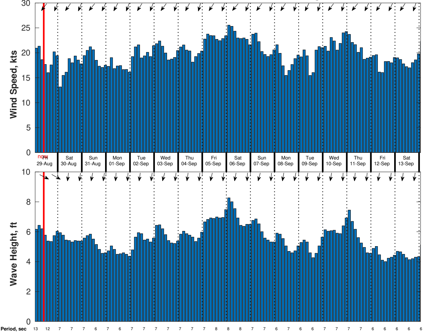
Wind & Wave Forecast for CSA (ONHYM) PPL EBS - Western Sahara from 28-Aug-2025 01:00:00 to 13-Sep-2025 01:00:00
