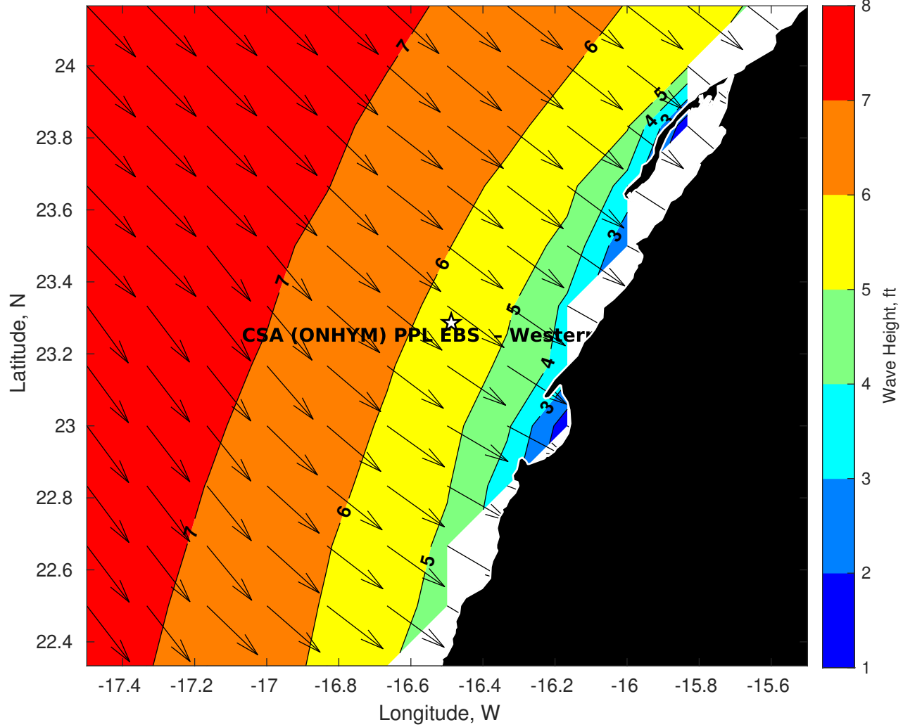
Wave Height (ft) for CSA (ONHYM) PPL EBS - Western Sahara at 28-Aug-2025 09:00:00
