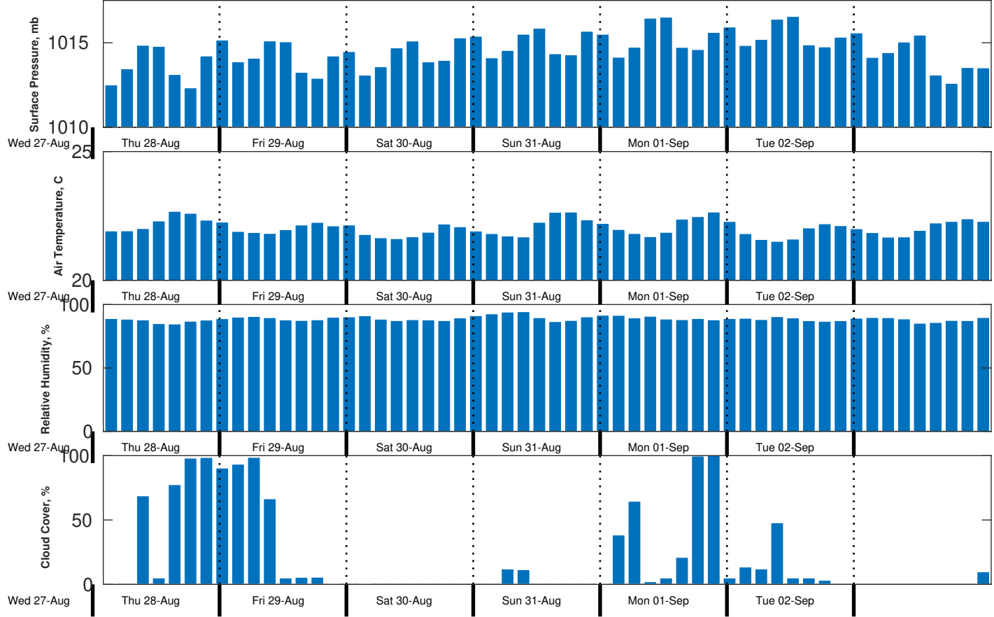
Met Forecast for CSA (ONHYM) PPL EBS - Western Sahara from 28-Aug-2025 00:00:00 to 04-Sep-2025 00:00:00
