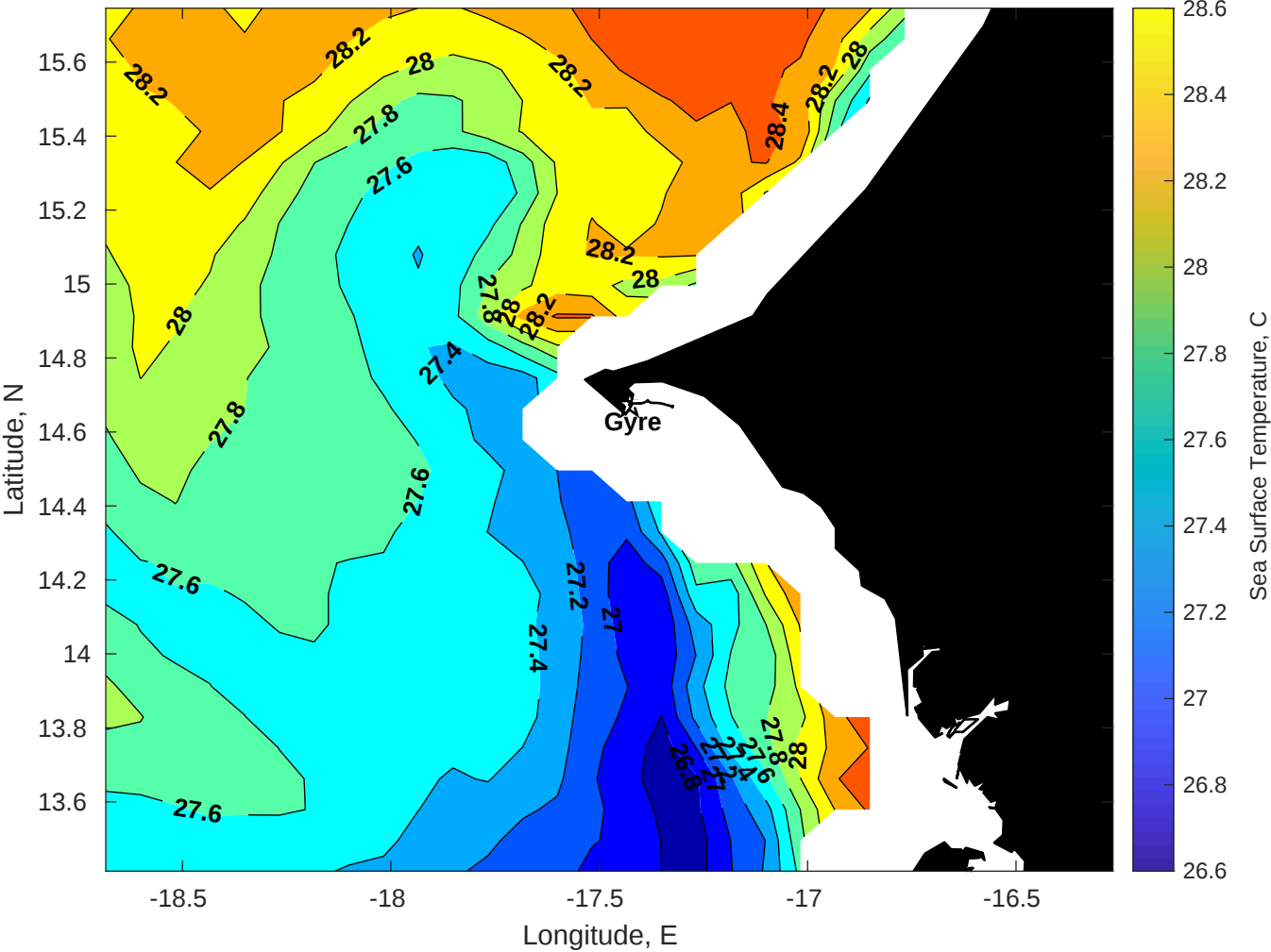
SST for Gyre at 27-Aug-2025 00:00:00
