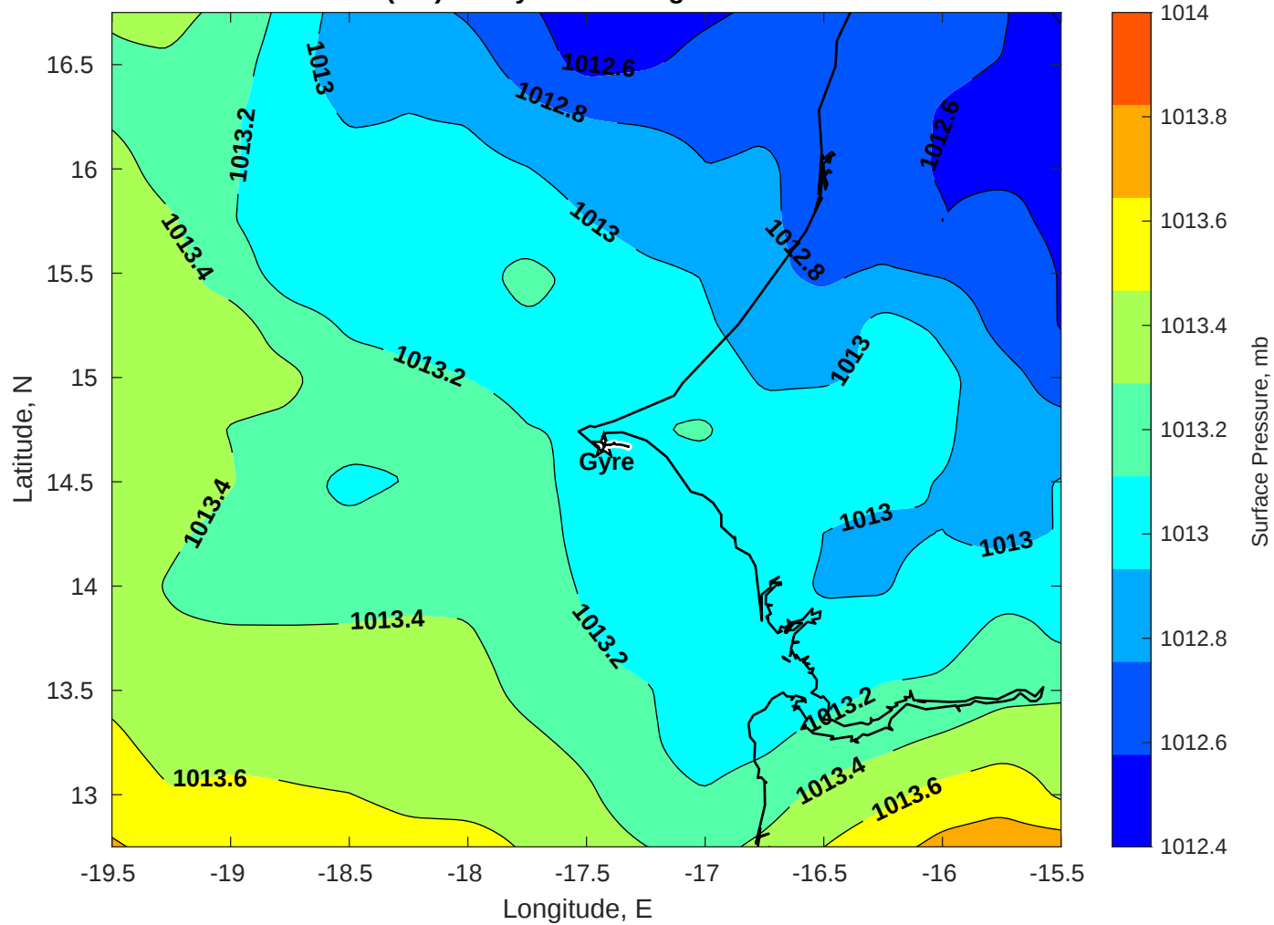
Surface Pressure (mb) for Gyre at 28-Aug-2025 00:00:00
