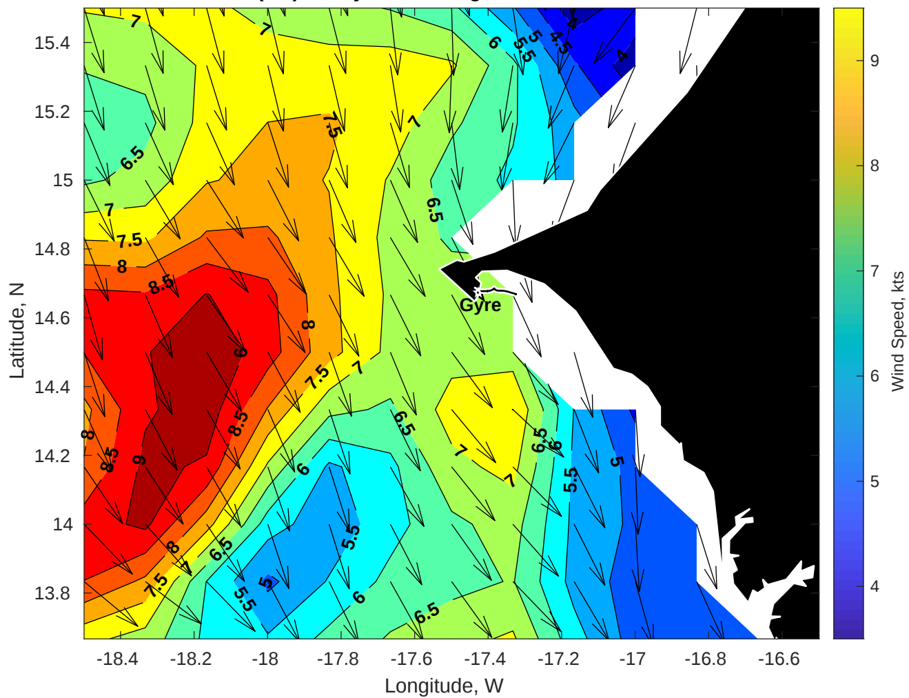
Winds (kts) for Gyre at 28-Aug-2025 09:00:00
