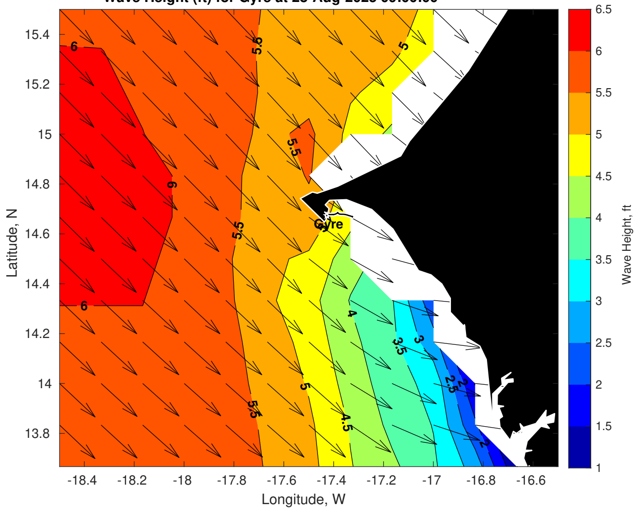
Wave Height (ft) for Gyre at 28-Aug-2025 09:00:00
