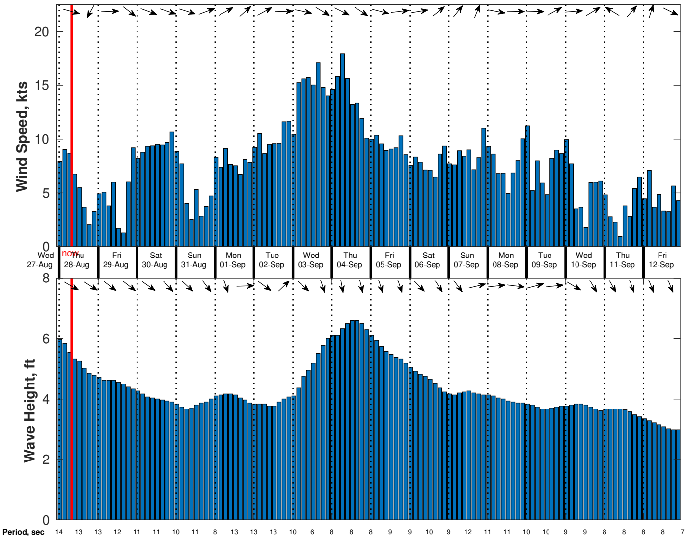
Wind & Wave Forecast for Gyre from 27-Aug-2025 23:00:00 to 12-Sep-2025 23:00:00
