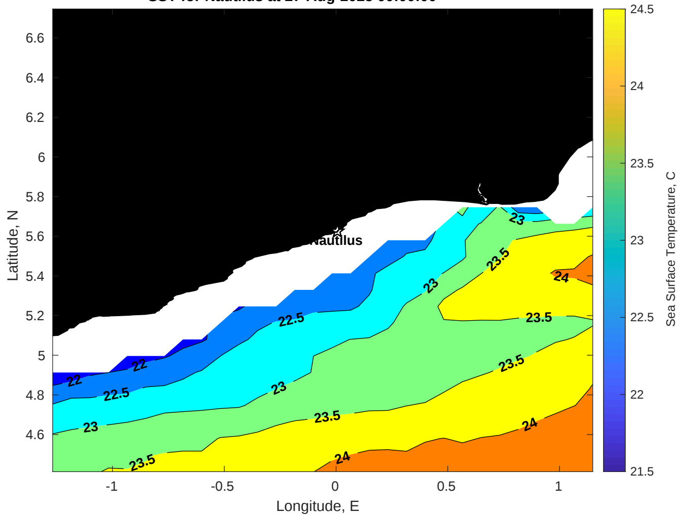
SST for Nautilus at 27-Aug-2025 00:00:00
