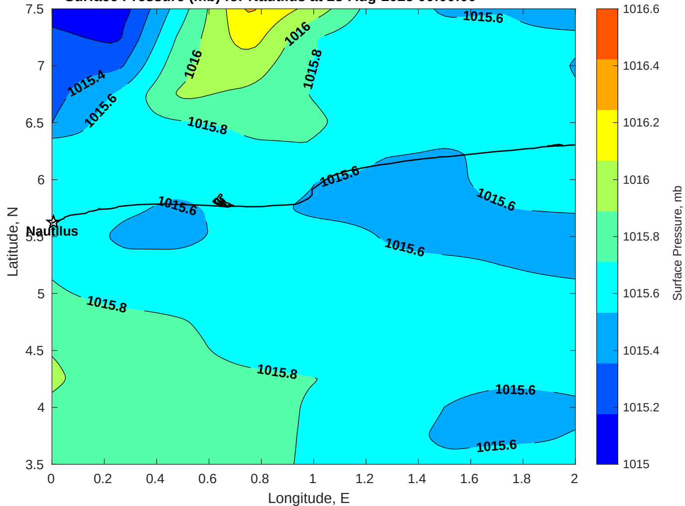
Surface Pressure (mb) for Nautilus at 28-Aug-2025 00:00:00
