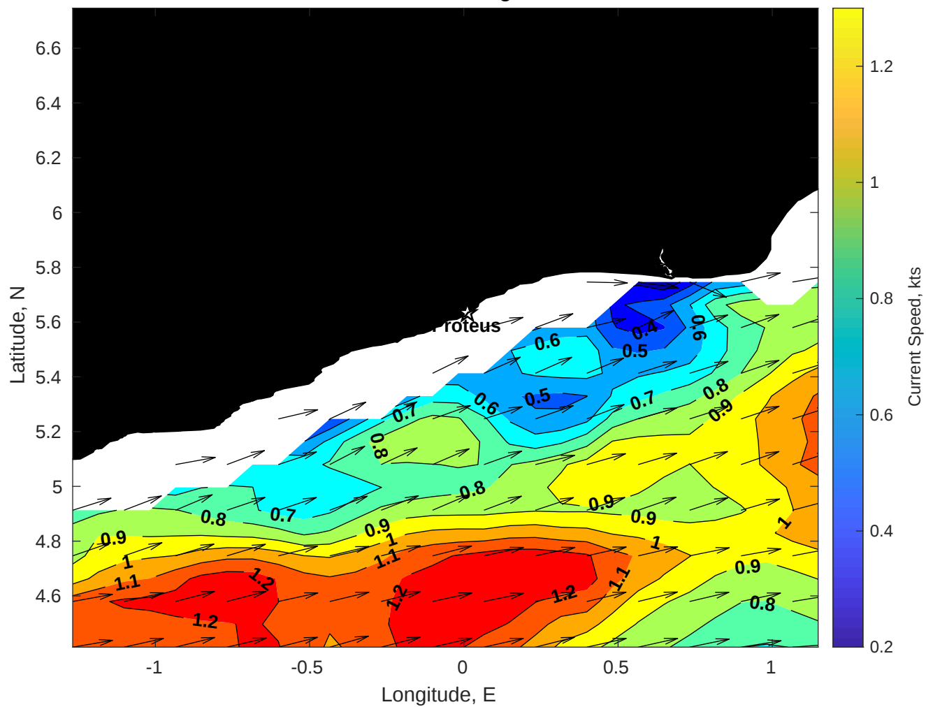
Surface Currents for Proteus at 27-Aug-2025 00:00:00
