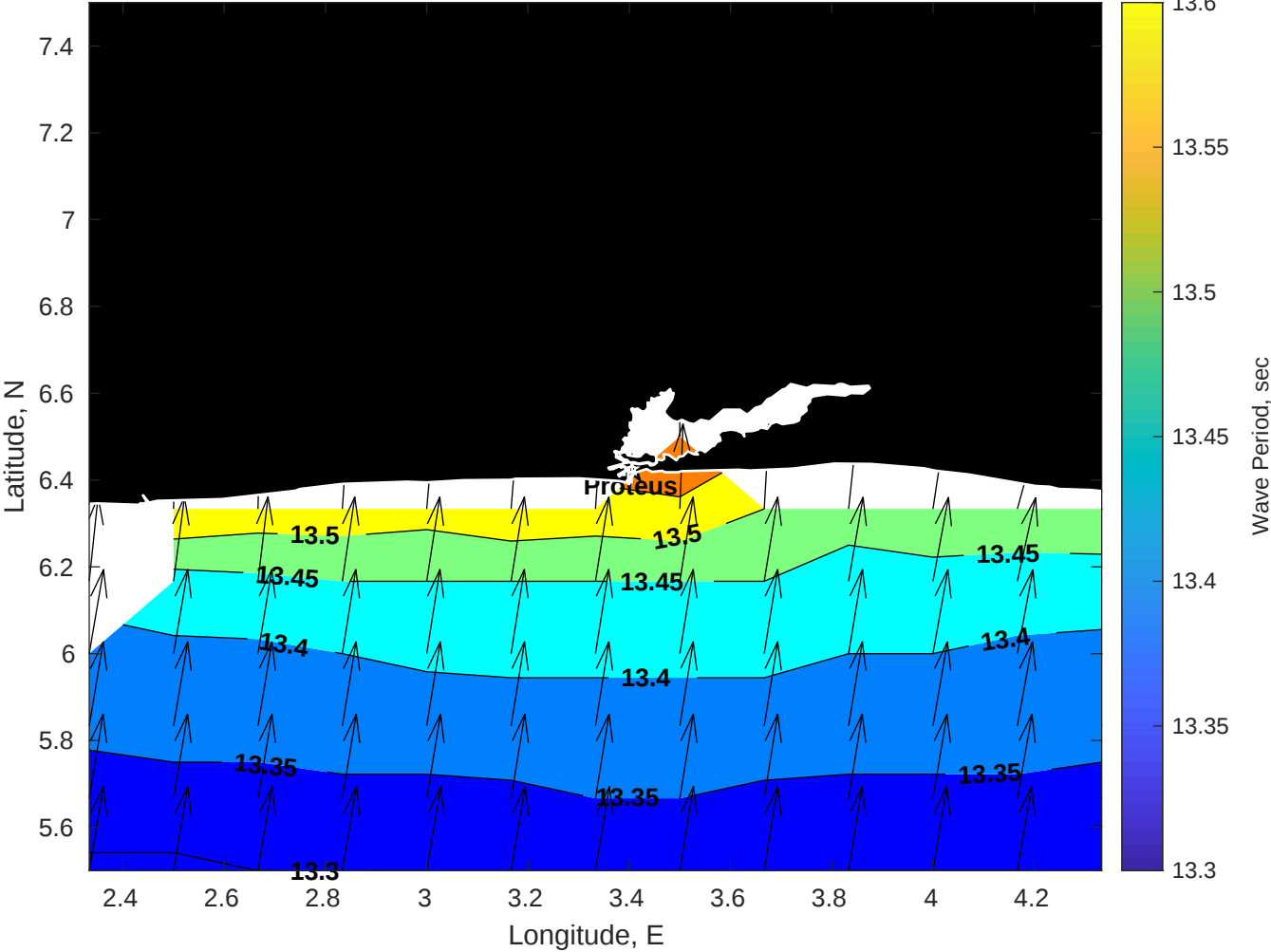
Wave Period (sec) for Proteus at 28-Aug-2025 09:00:00
