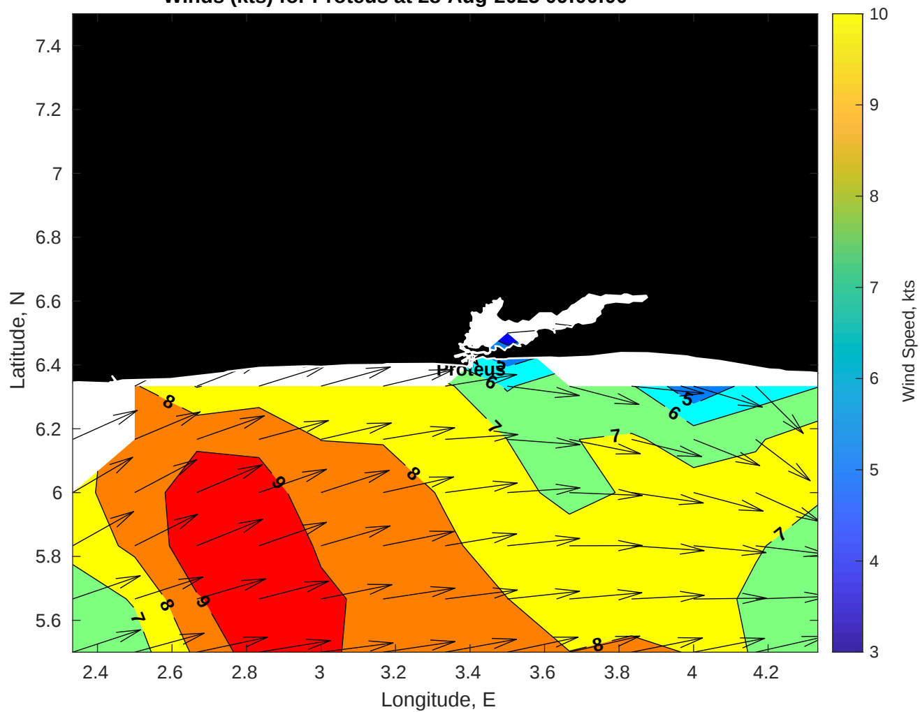
Winds (kts) for Proteus at 28-Aug-2025 09:00:00
